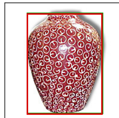
vase IoU 0.98
