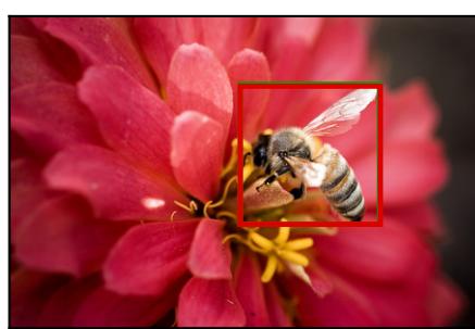
bee IoU 0.98
