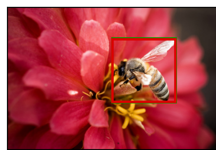
bee IoU 0.97
