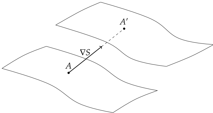
Figure 2: Displacement of a constant action surface after a time interval \delta t .
