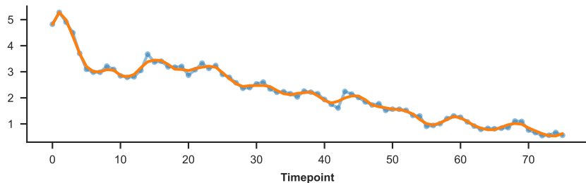
Polarity Magnitude
