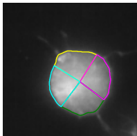
Polarity Magnitude
