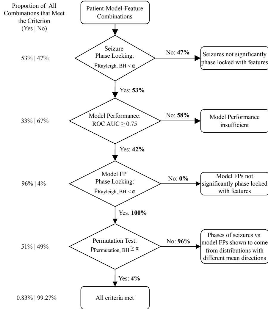
Figure 3.1: Proportions of Patient-Model-Feature Combinations that Met each Criterion.
