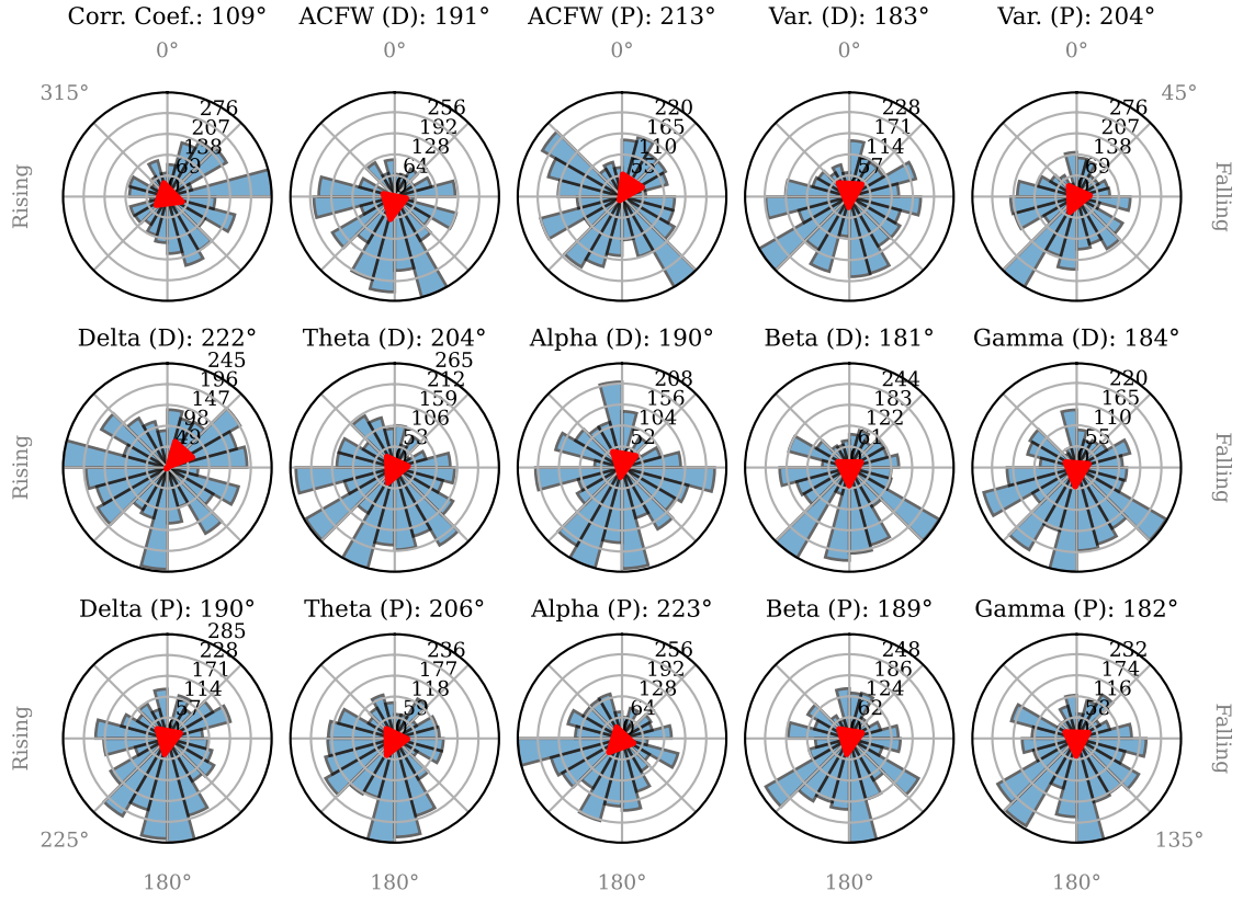
Figure 3.7: CNN FP Phase Histogram per Feature of Patient C03
