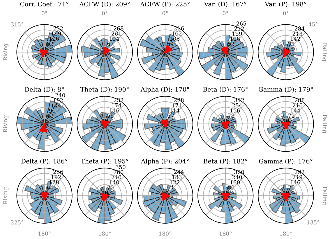
Figure 3.8: Ensemble FP Phase Histogram per Feature of Patient C03
