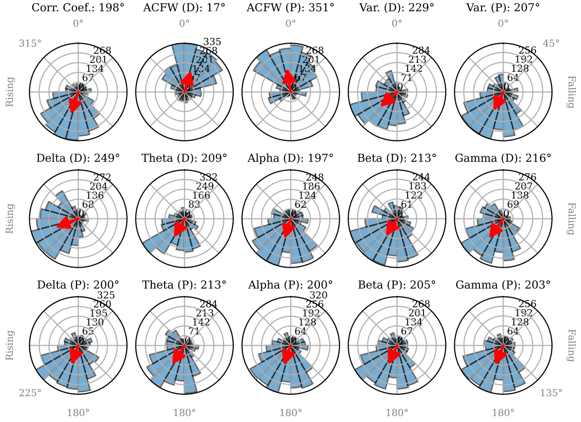
Figure 3.4: Ensemble FP Phase Histogram per Feature of Patient U01
