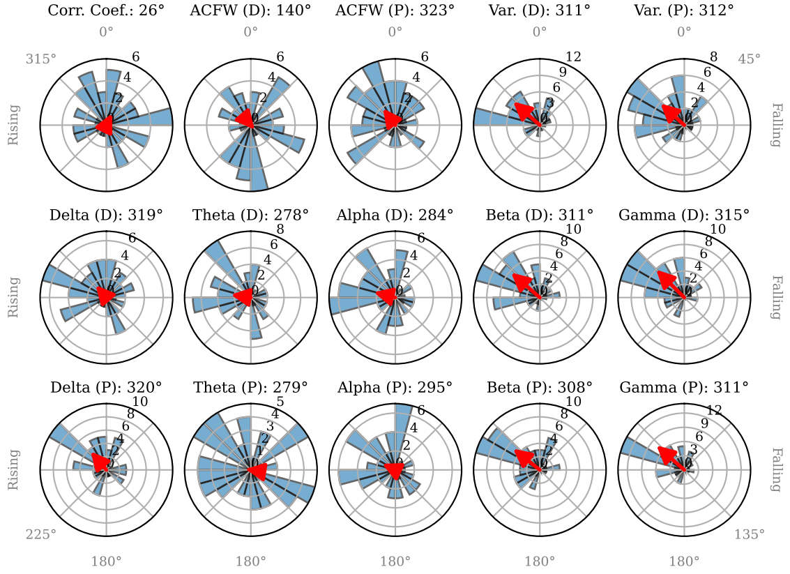
Figure 3.6: Seizure Phase Histogram per Feature of Patient C03.
