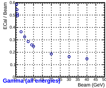
Beam VS ECAL/Beam
