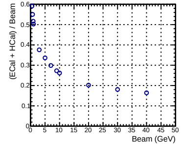
Beam VS (ECAL + HCAL)/Beam
