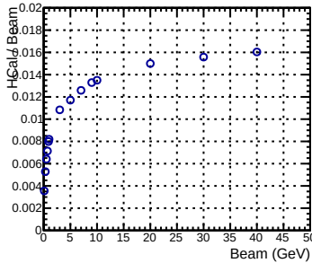
Beam VS HCAL/Beam
