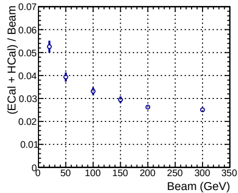
Neutron: Beam VS (ECAL + HCAL)/Beam
