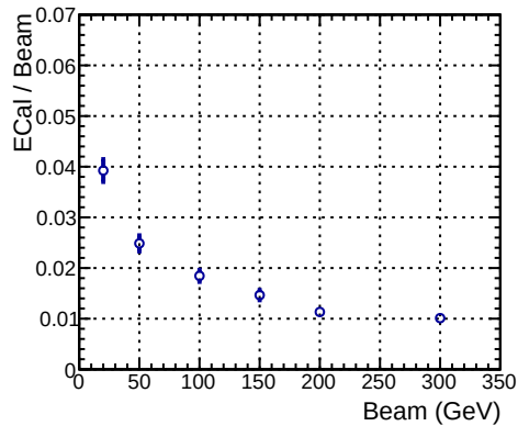
Neutron: Beam VS ECAL/Beam
