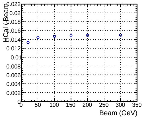
Neutron: Beam VS HCAL/Beam
