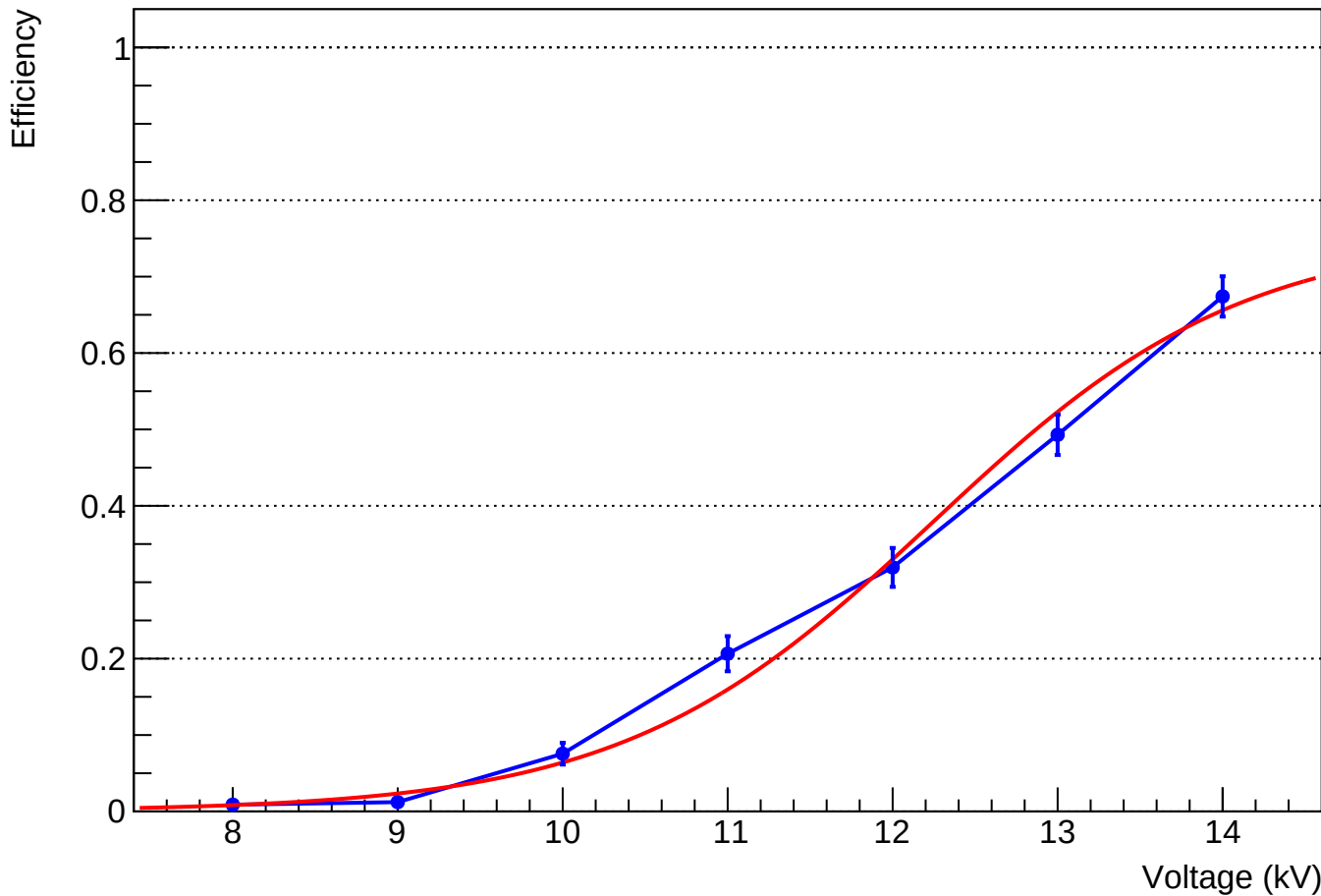
Efficiency vs Voltage
