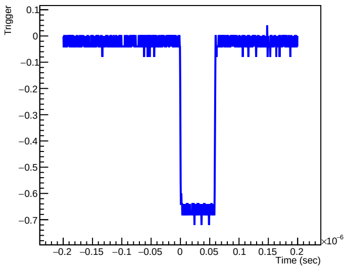
Trigger vs Time
