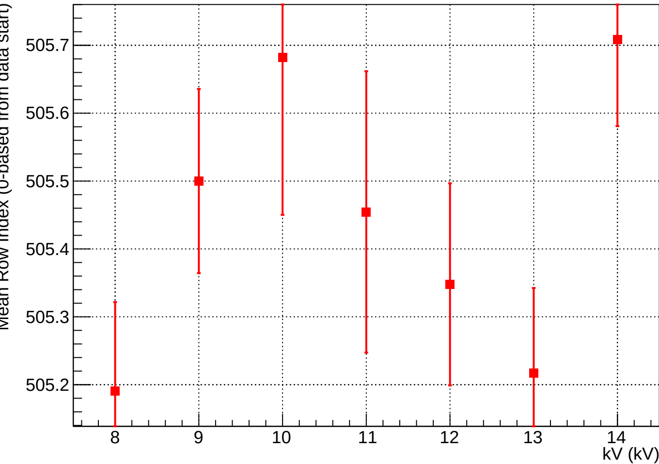
Mean Row Index of 2nd Crossing vs kV
