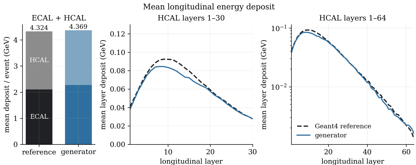
Figure 3: Mean deposited energy over all 10,000 development-bank events. Left: ECAL and HCAL deposits expose section-level compensation. Center: HCAL layers 1–30 (linear scale). Right: HCAL layers 1–64 (log scale). Dashed curves denote Geant4, solid curves the generator; ECAL layer 0 enters only the bars. Event averages include empty showers and do not resolve individual interior gaps.
