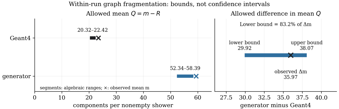
Figure 4: Graph fragmentation conditional on nonempty readout (9,907 Geant4 and 9,858 generated showers). Left: observed mean component counts m (crosses) and allowed ranges of Q = m - R (segments). Right: the allowed difference in mean Q compared with the observed difference in mean m . Ranges follow from 1 \leq R \leq G + 1 ; they are algebraic bounds, not uncertainty intervals. All quantities use strictly positive deposits and the model graph.
