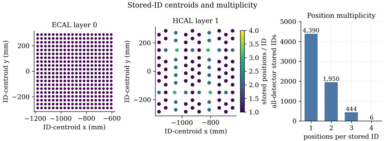
Figure 1: Stored-ID geometry: ECAL layer 0, HCAL layer 1, and position multiplicity over all 6,790 IDs. The first bar contains 400 ECAL and 3,990 HCAL IDs. Centroids define model nodes; multiplicity does not verify physical readout ganging.
