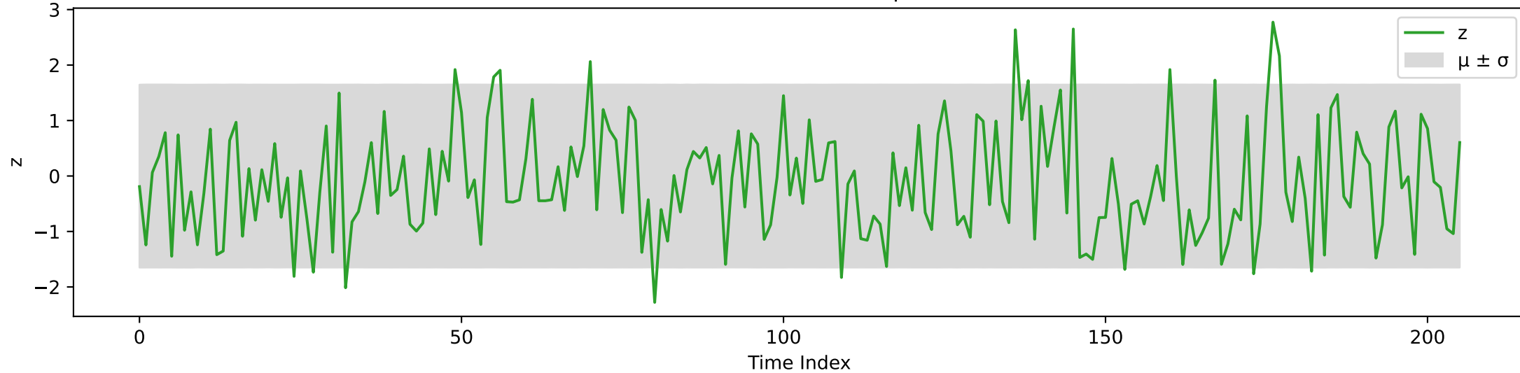
MIMO-VAE: Latent Sample ( z )
