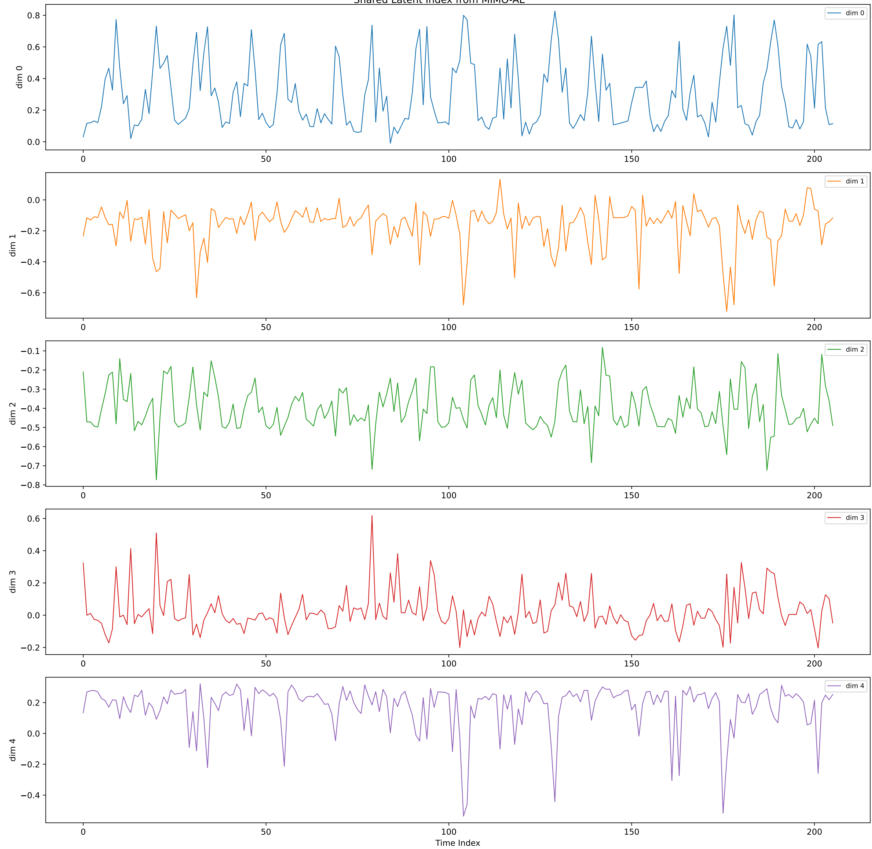
Shared Latent Index from MIMO-AE
