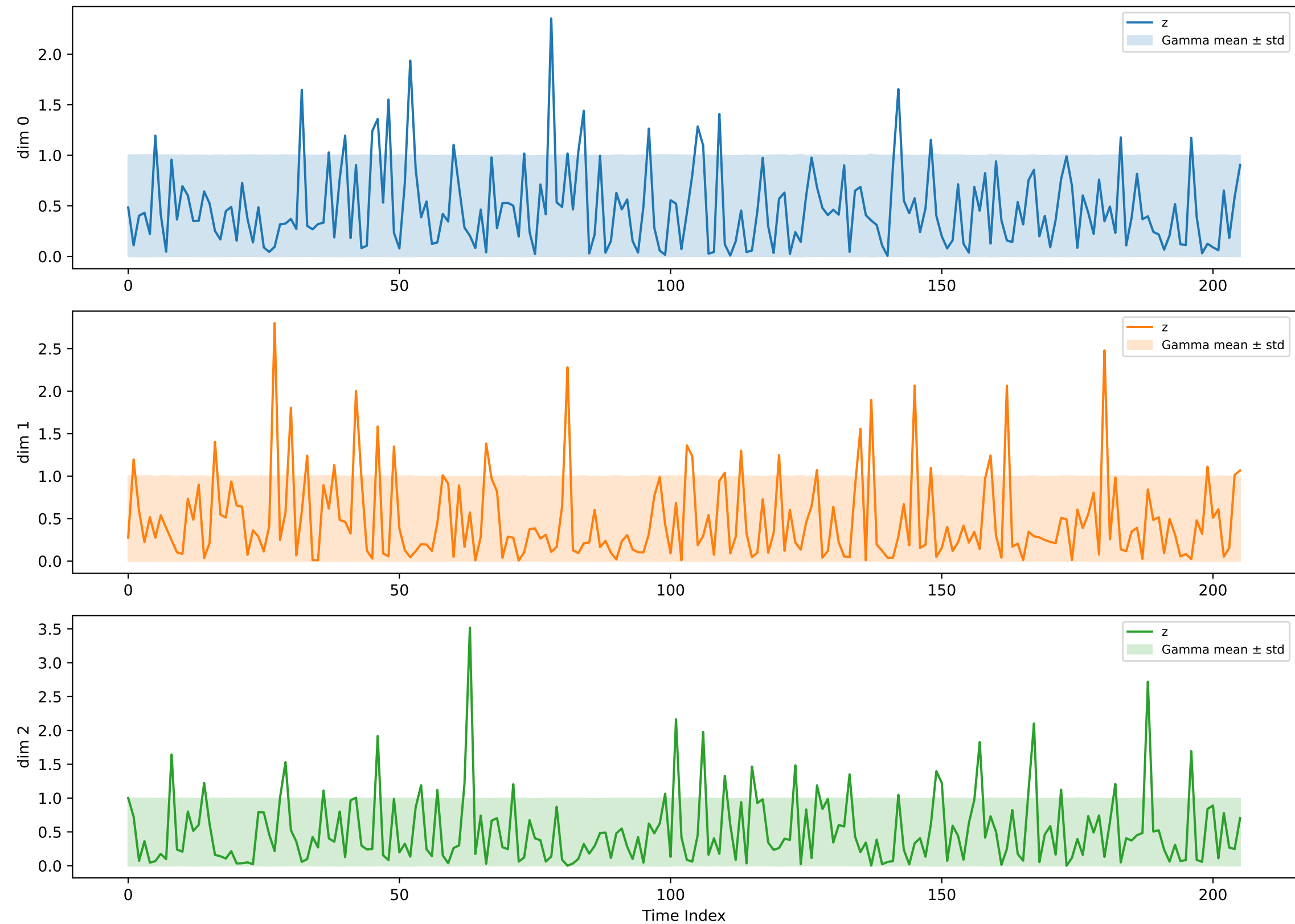
MIMO-VAE (Gamma Latent): Latent Sample (z)
