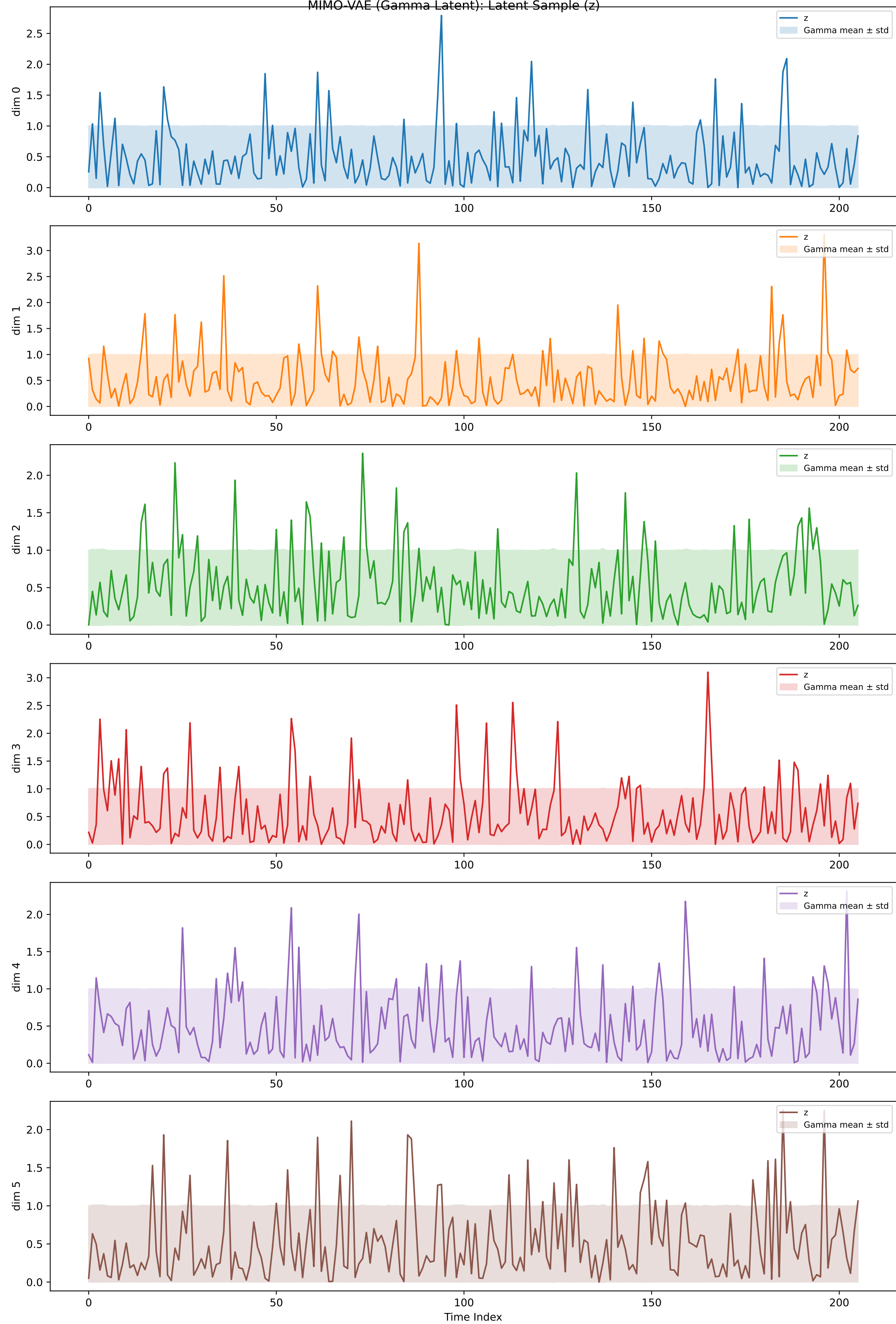
MIMO-VAE (Gamma Latent): Latent Sample (z)
