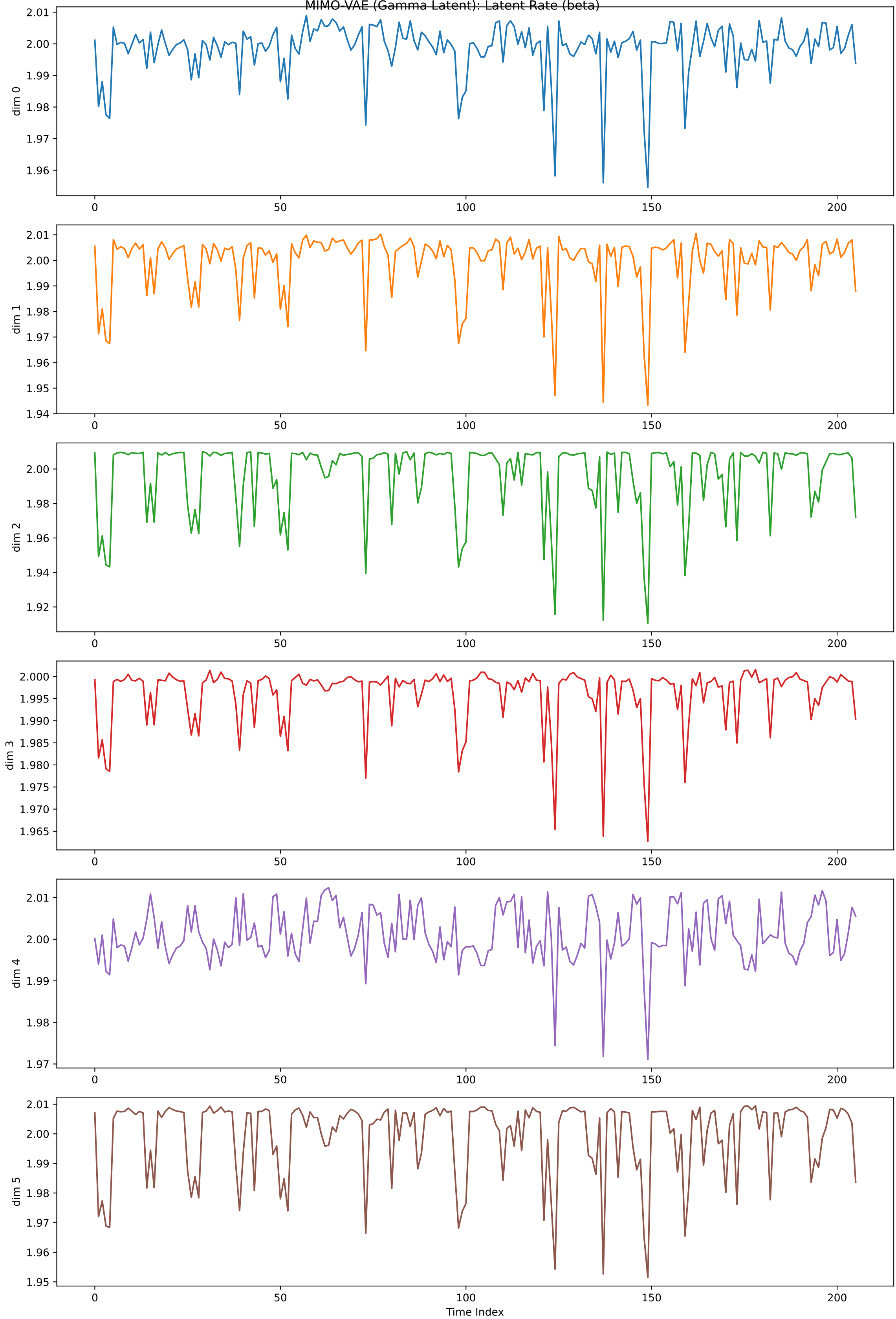
MIMO-VAE (Gamma Latent): Latent Rate ( \beta )
