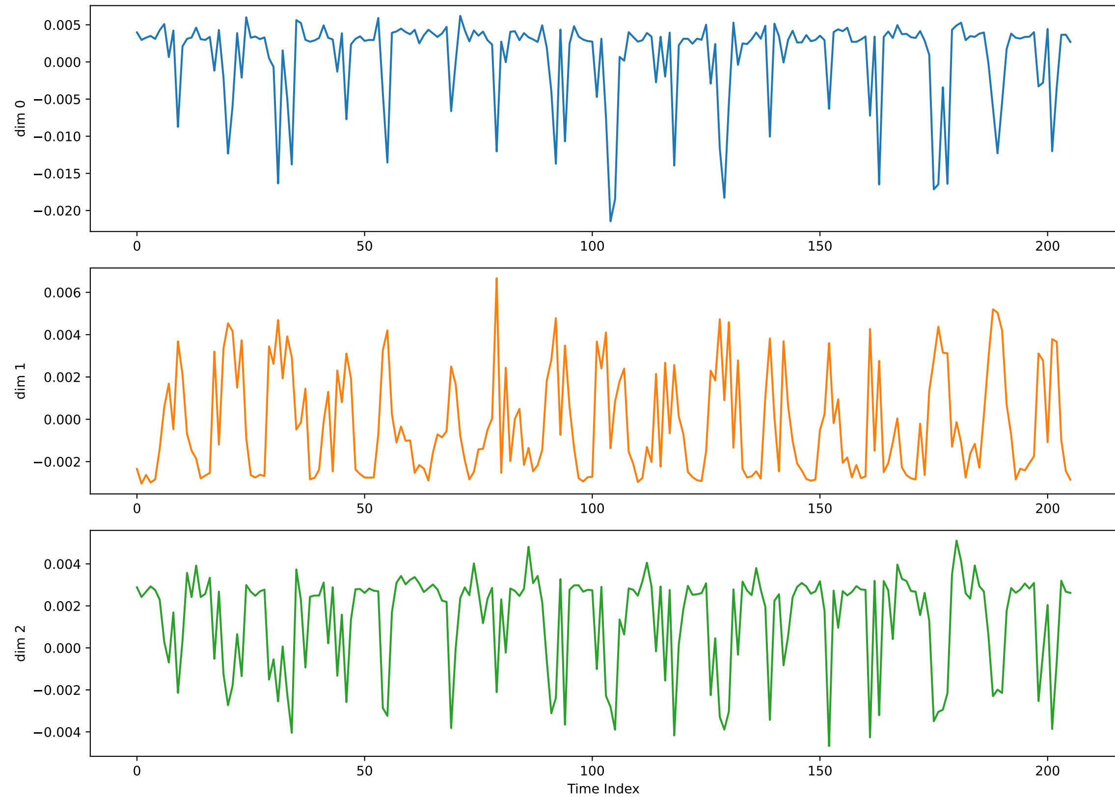
MIMO-VAE: Latent Mean ( \mu )
