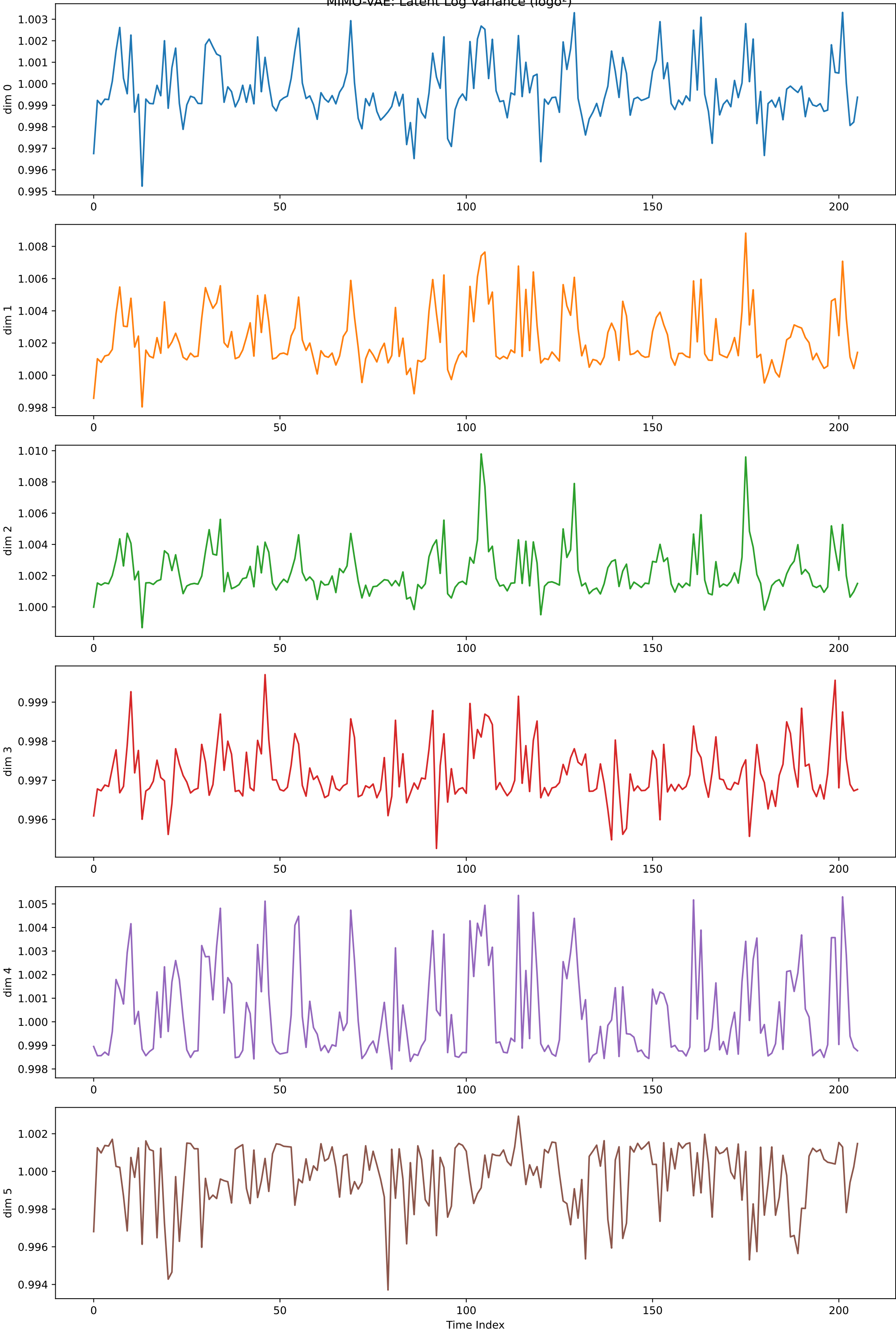
MIMO-VAE: Latent Log Variance ( \log \sigma^2 )
