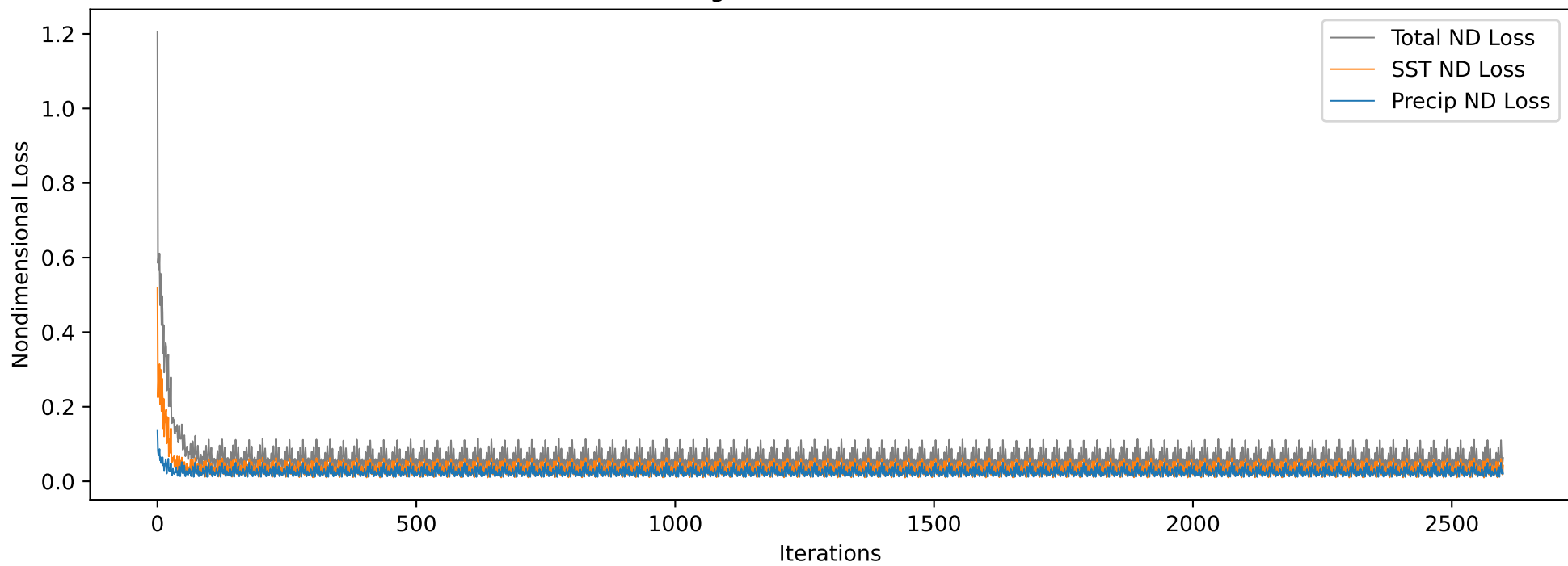
Training Nondimensional Losses
