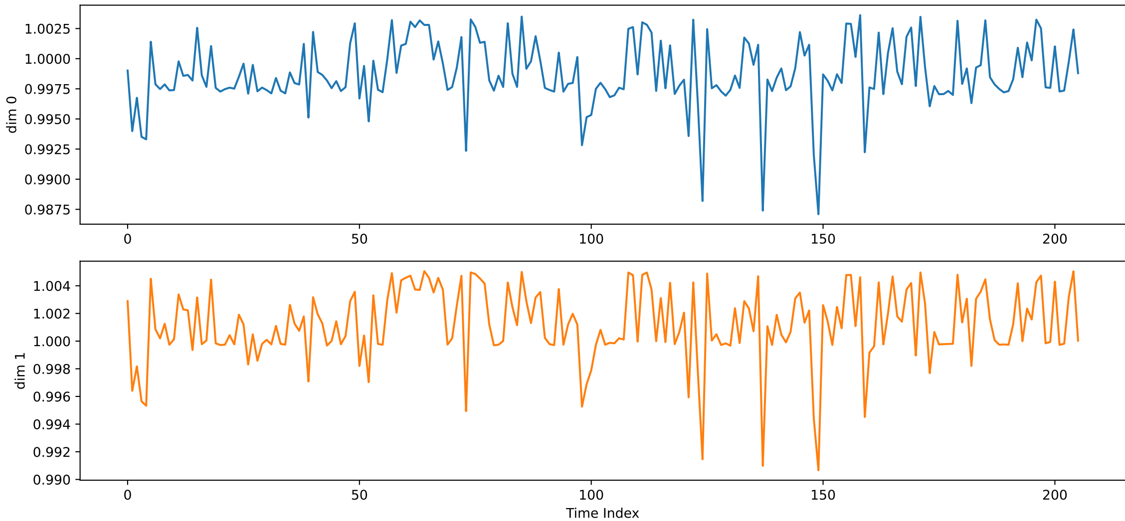
MIMO-VAE (Gamma Latent): Latent Shape ( \alpha )
