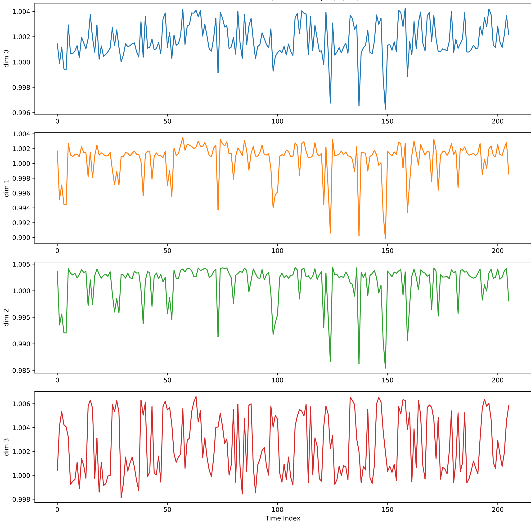
MIMO-VAE (Gamma Latent): Latent Shape (alpha)
