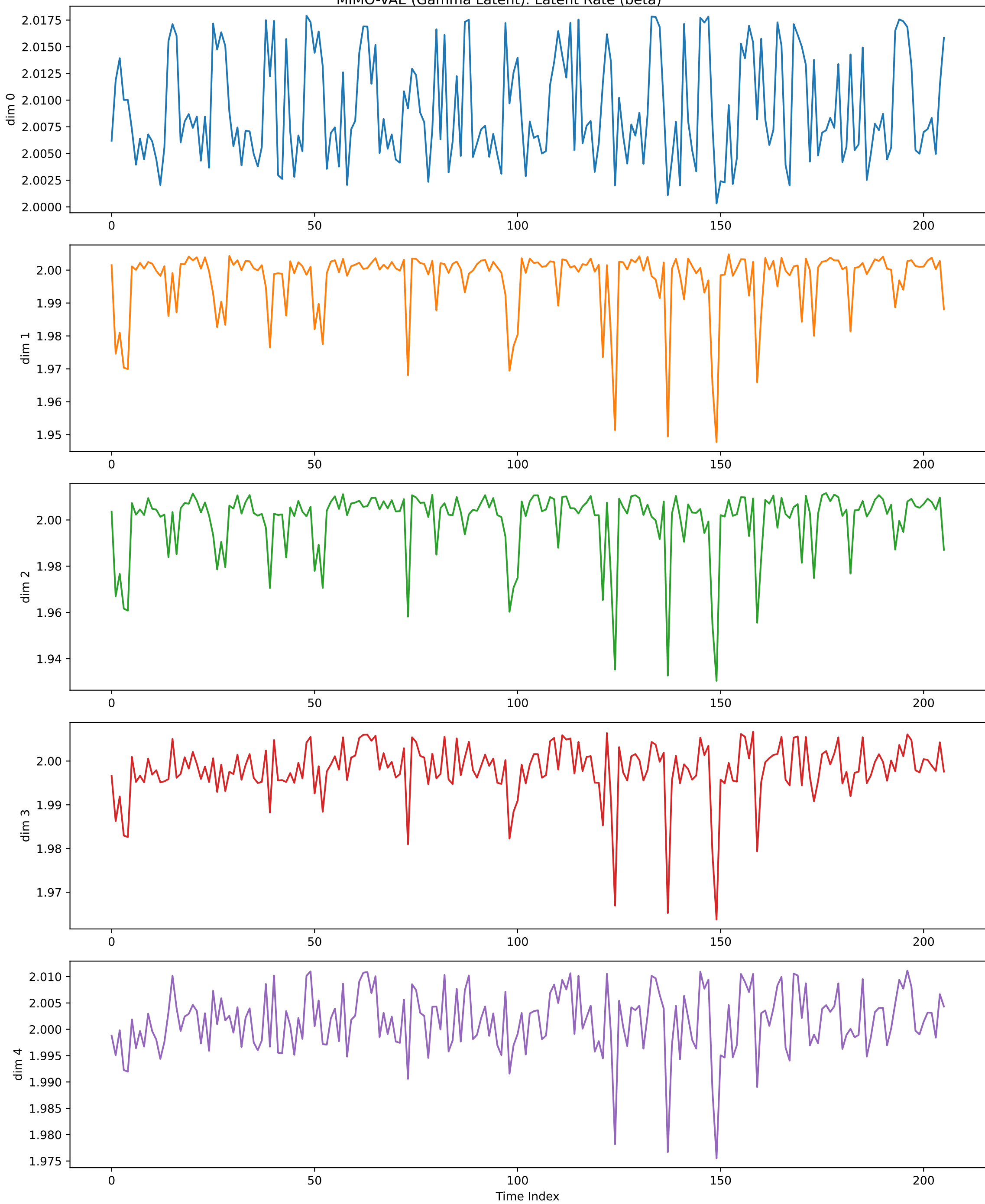
MIMO-VAE (Gamma Latent): Latent Rate ( \beta )
