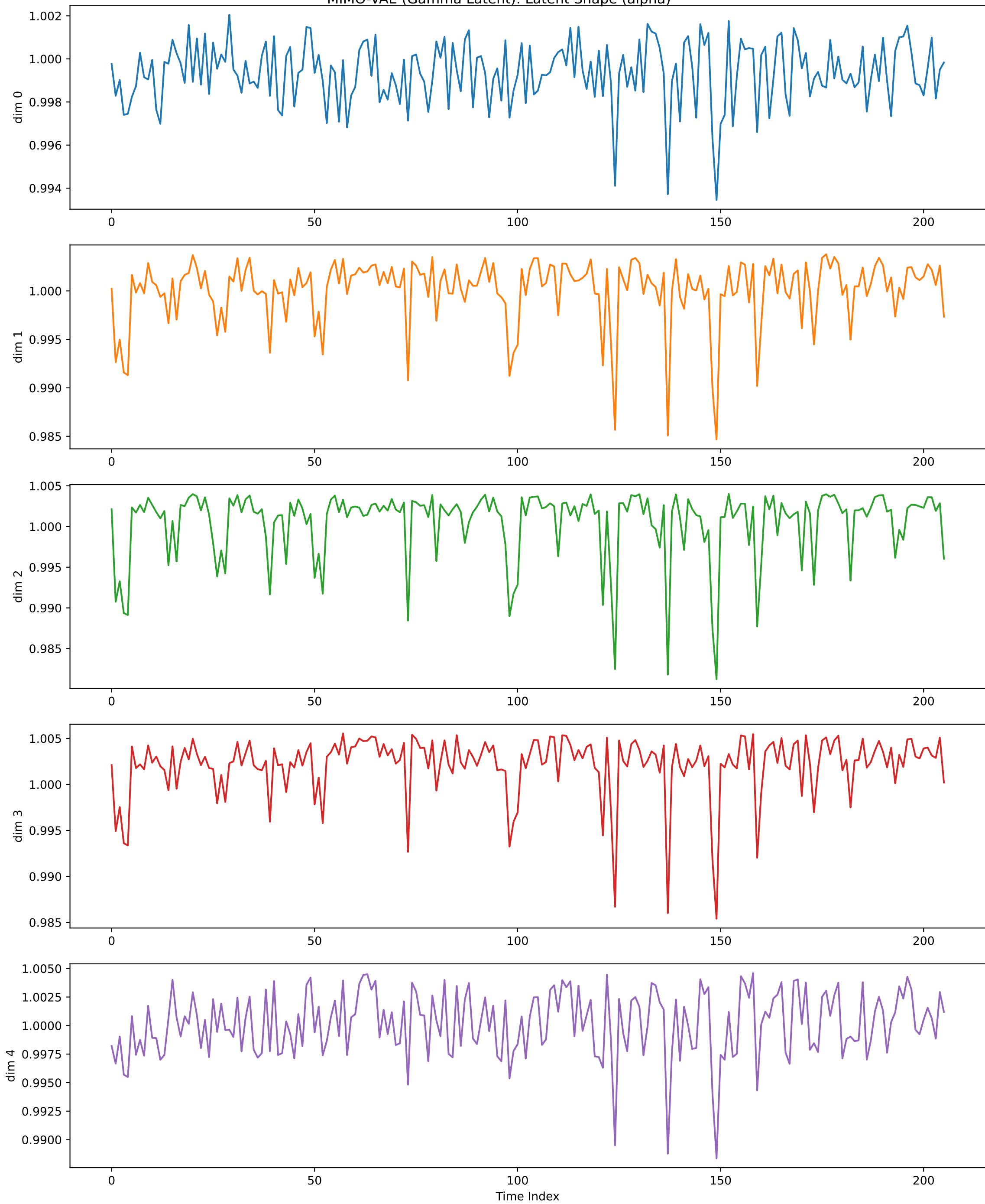
MIMO-VAE (Gamma Latent): Latent Shape (alpha)
