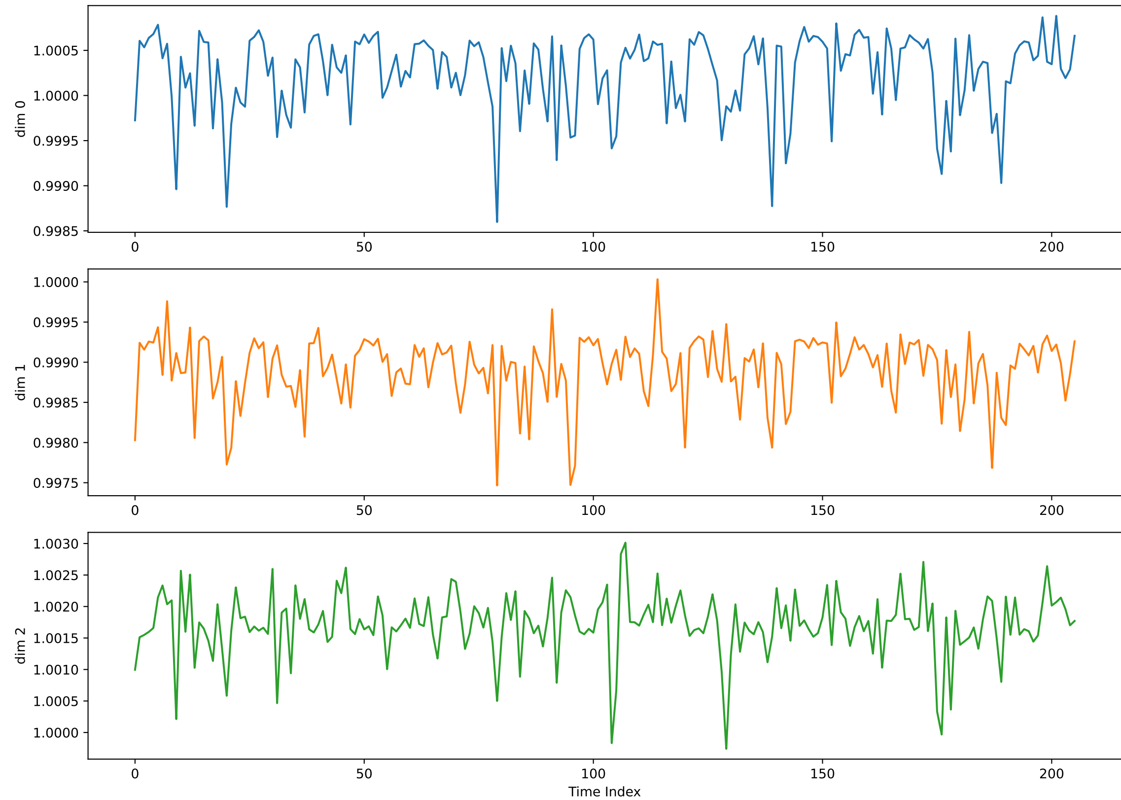
MIMO-VAE: Latent Log Variance ( \log\sigma^2 )
