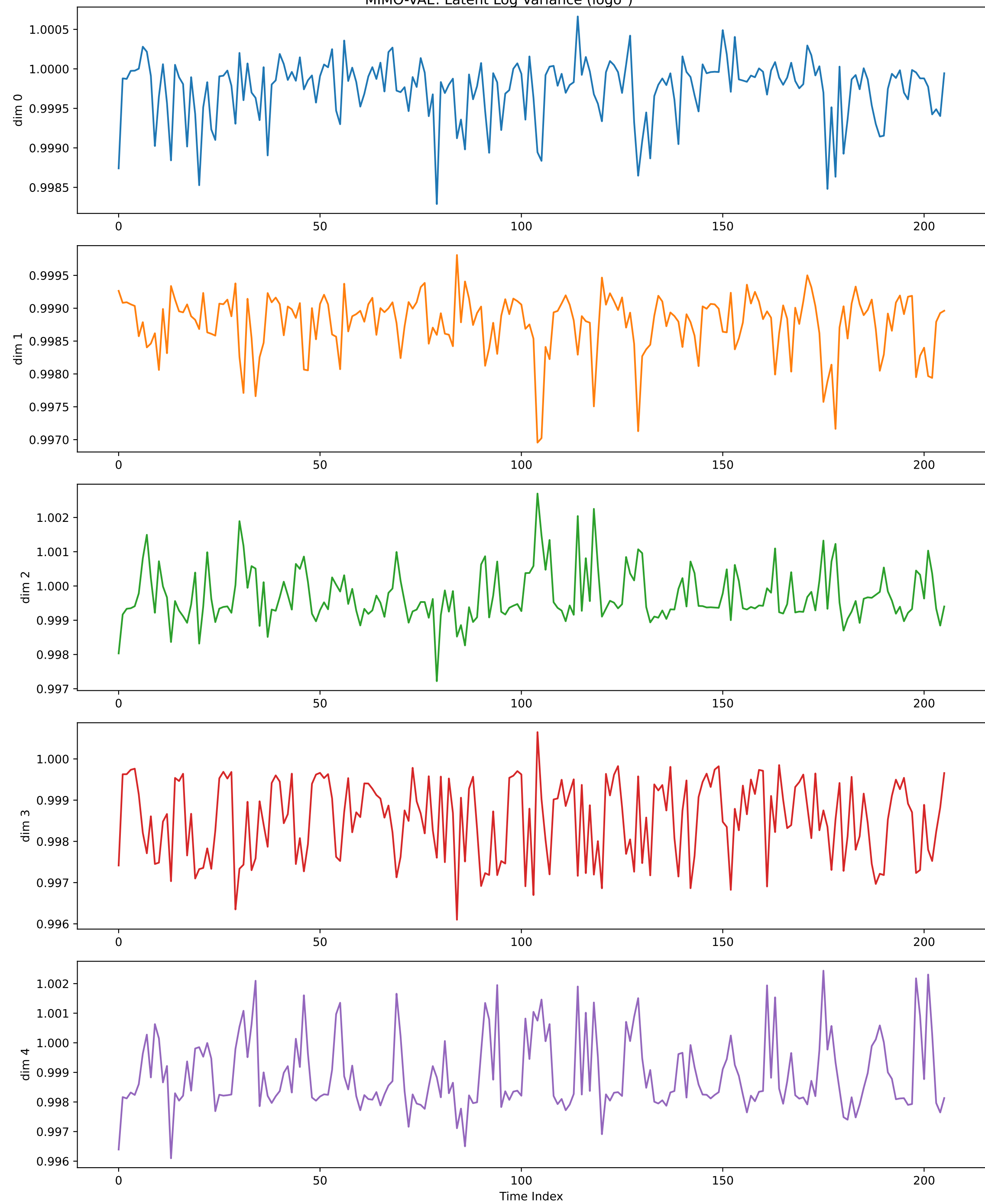
MIMO-VAE: Latent Log Variance ( \log \sigma^2 )
