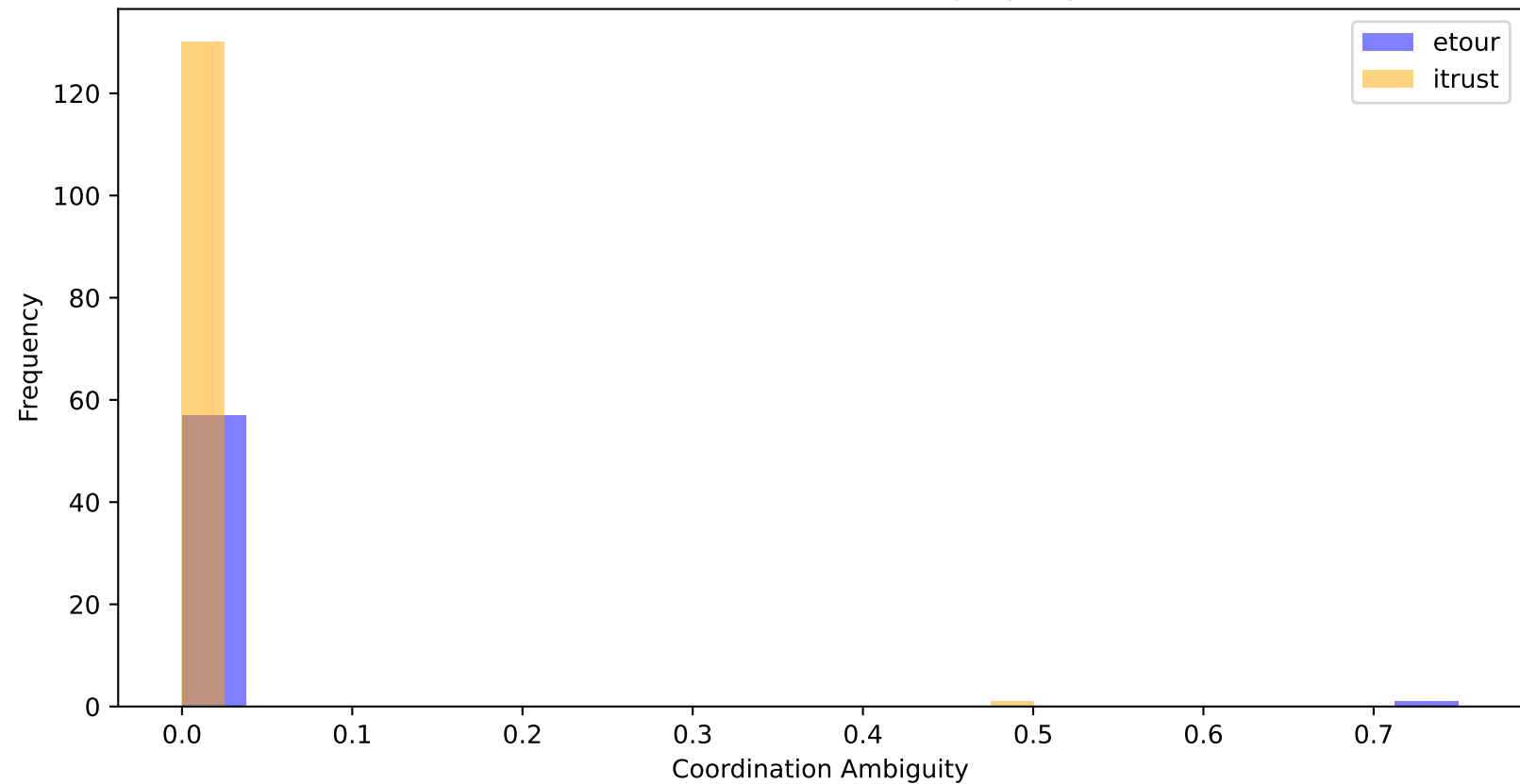
Distribution of "Coordination Ambiguity" by Dataset
