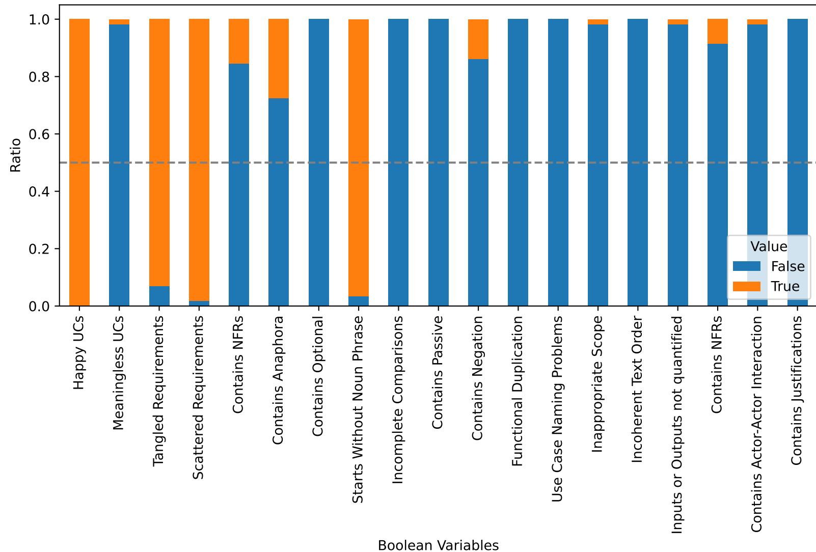
Ratio of False to True for Boolean Variables in etour
