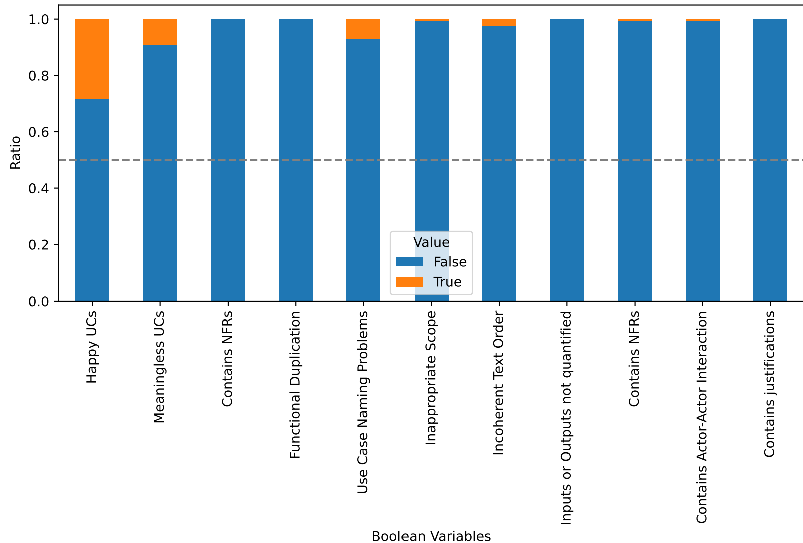
Ratio of False to True for Boolean Variables in itrust
