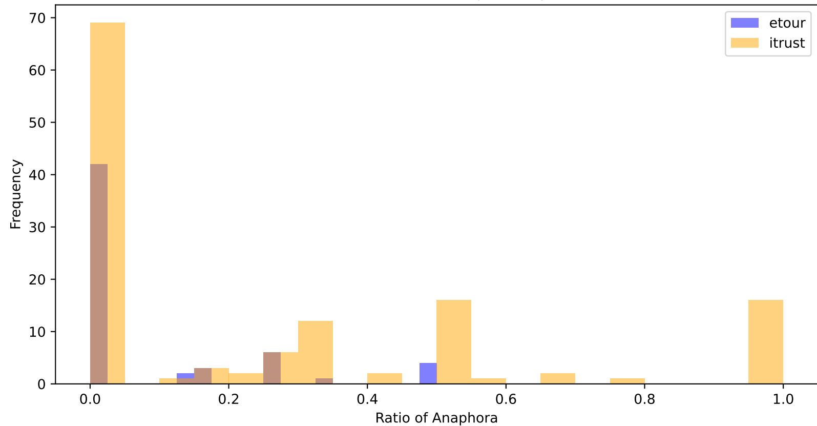
Distribution of Ratio of Anaphora by Dataset
