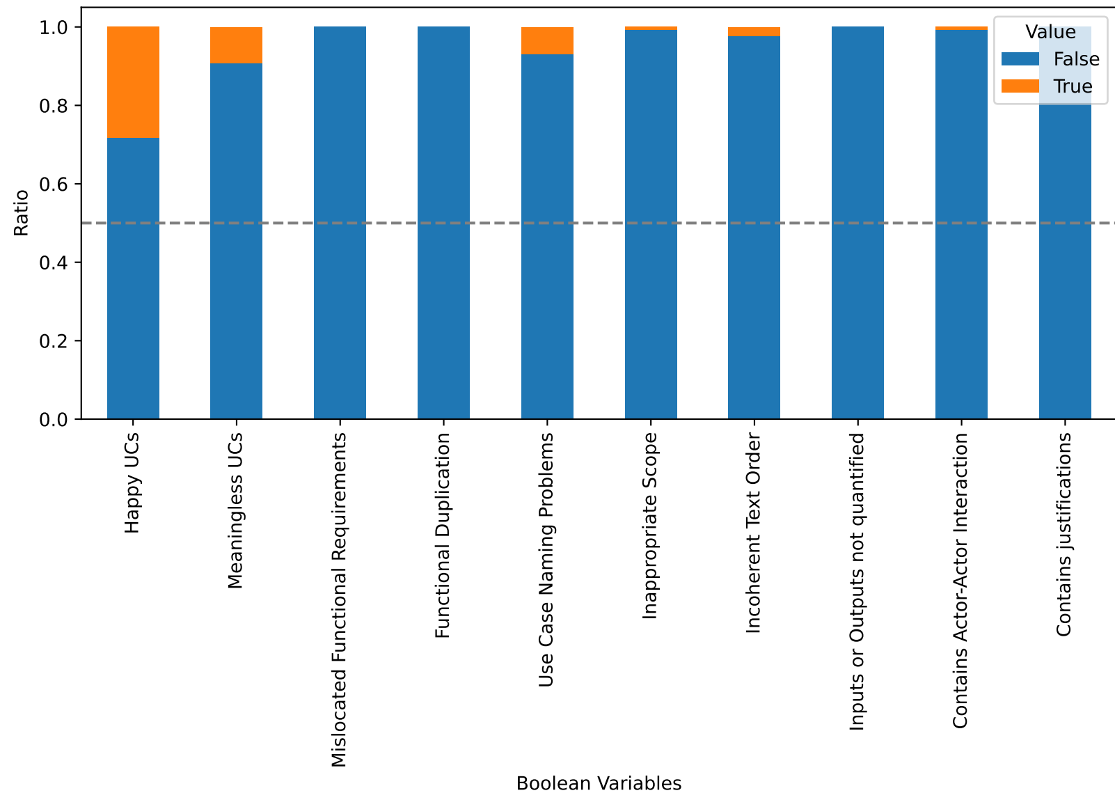
Ratio of False to True for Boolean Variables in itrust
