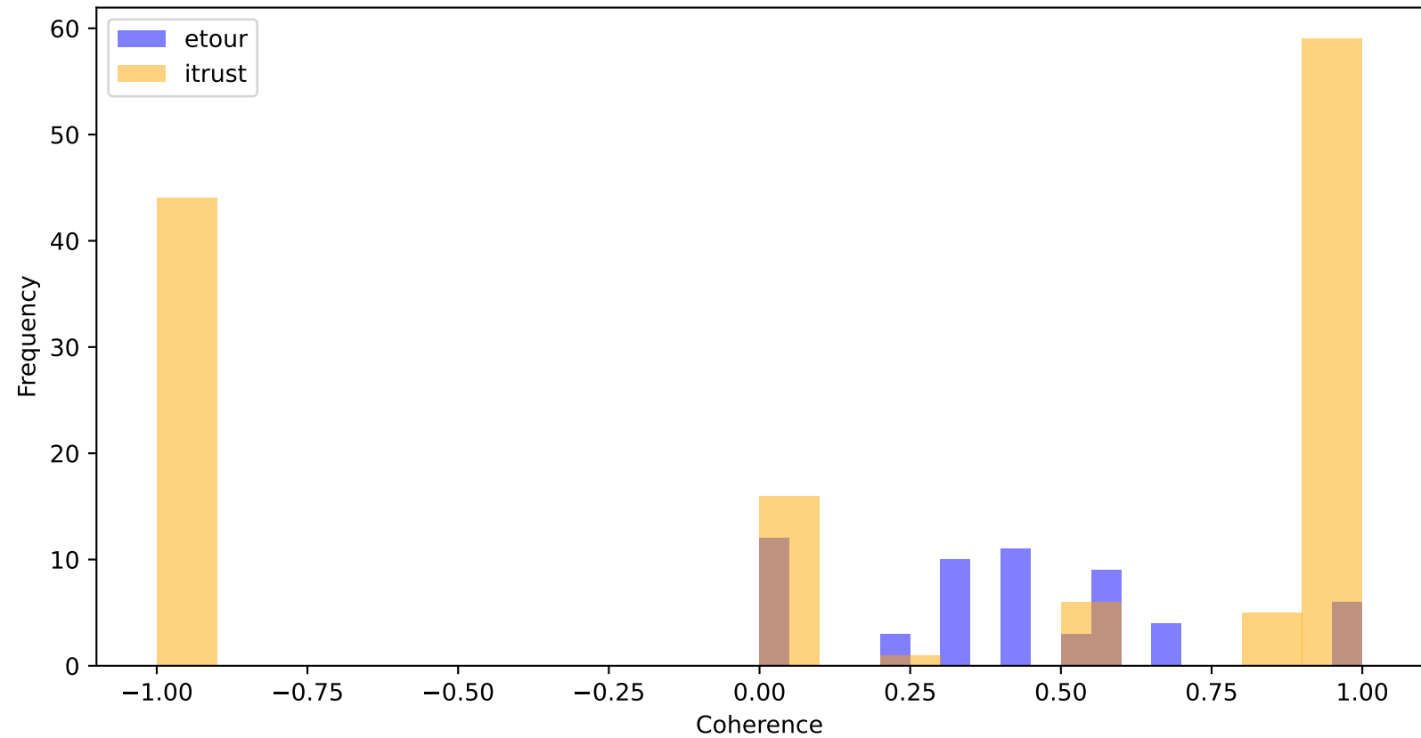
Distribution of Coherence by Dataset
