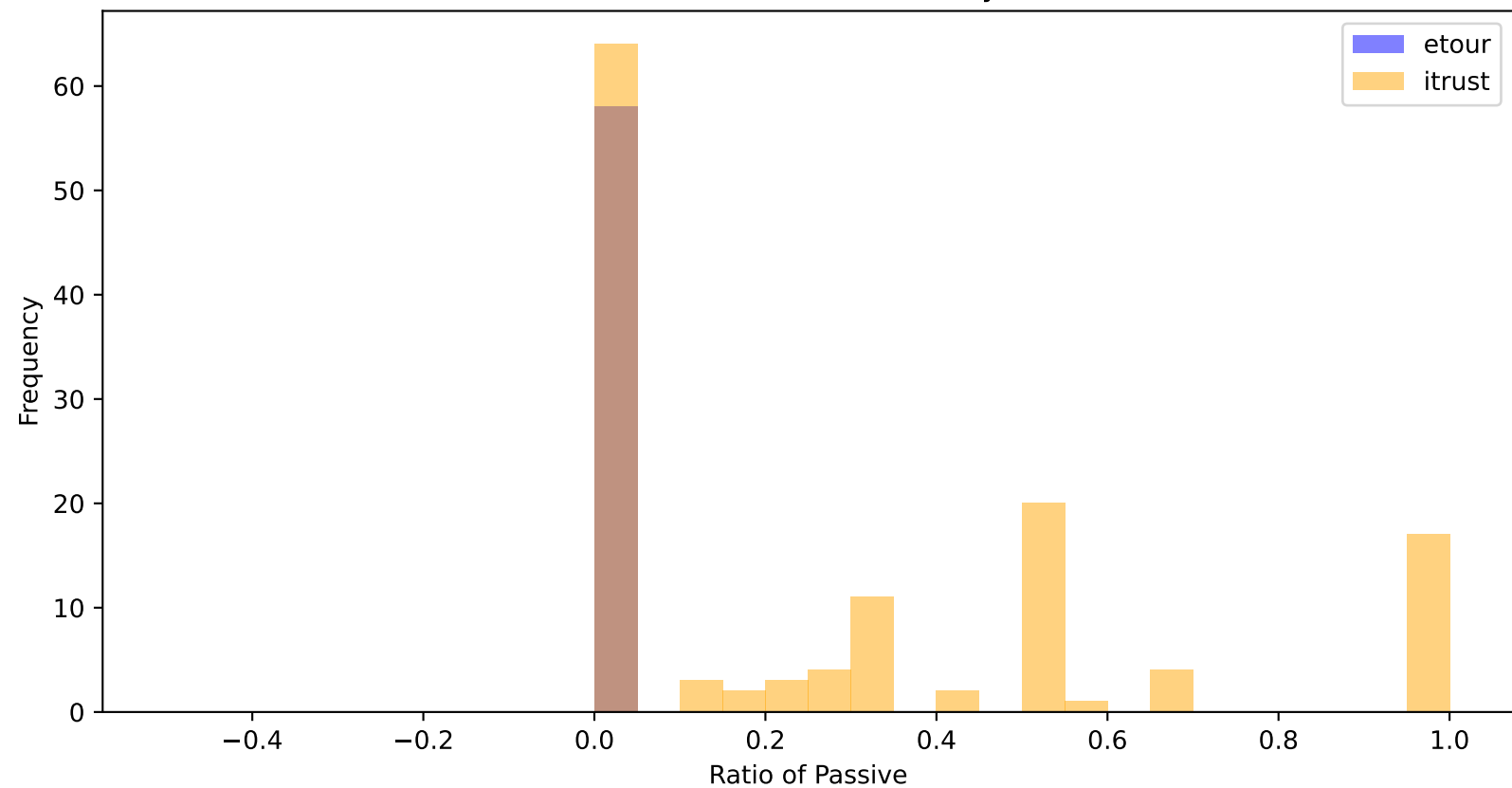
Distribution of Ratio of Passive by Dataset
