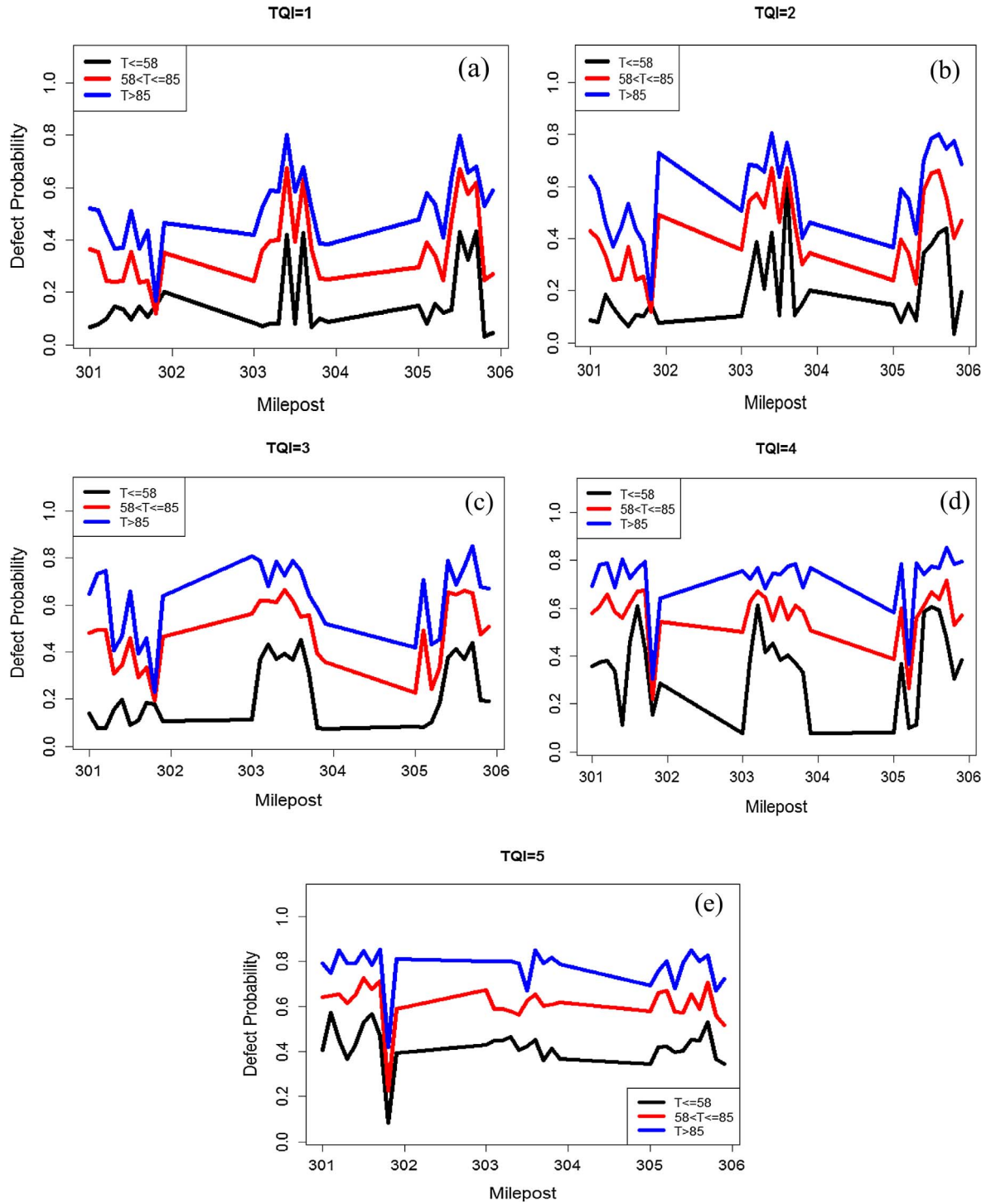
Fig. 5. The occurrence probability of geo-defects under different inspection intervals for five TQI levels; (a)–(e) represents TQI levels 1–5, respectively.
