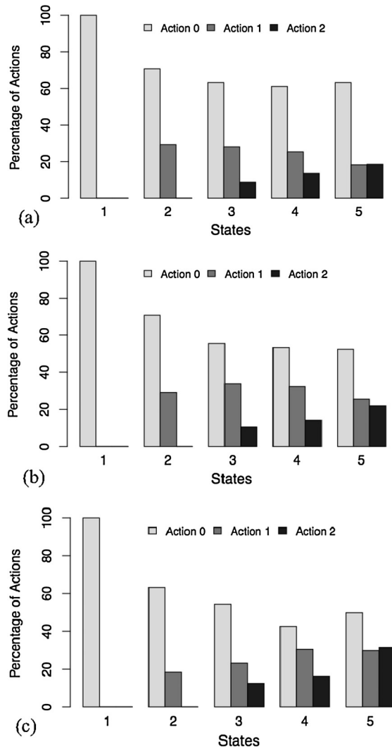
Fig. 9. Existing policy as derived from actual data for (a) T = 0-58 days (b) T = 59-85 days (c) T > 85 days.
