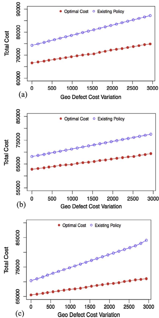
Fig. 15. Sensitivity analysis of geo-defect corrective maintenance cost for (a) T < 58 days (b) T = 59-85 days (c) T > 85 days.
