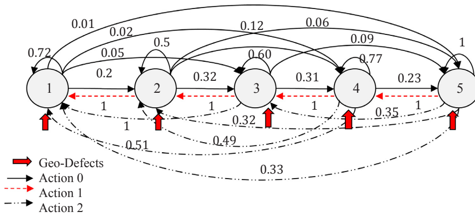
Fig. 8. The proposed MDP with 5 states and 3 actions for the inspection interval 0–58 days.
