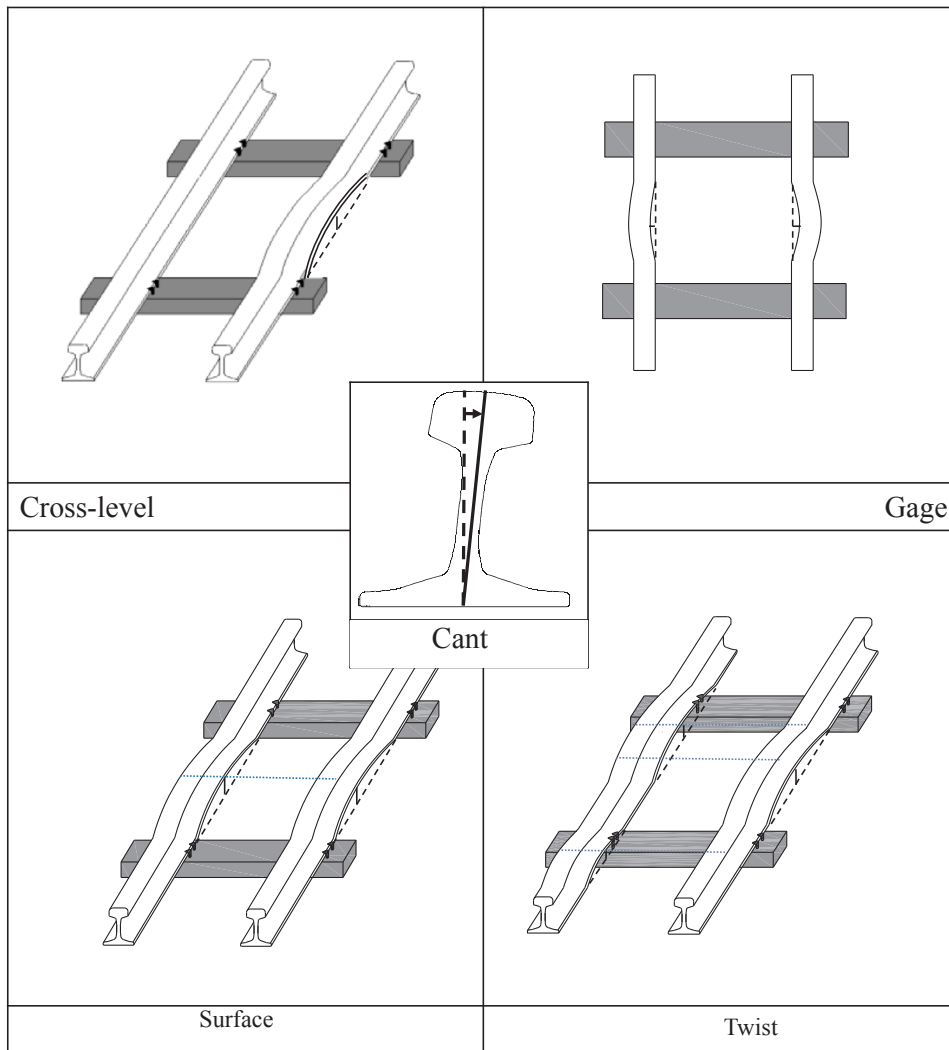
Fig. 1. Track geometry measurements.
