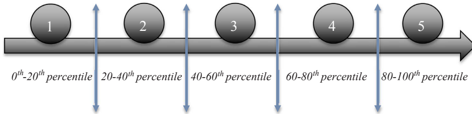
Fig. 7. Determination of the Markov chain states based on TQI values.
