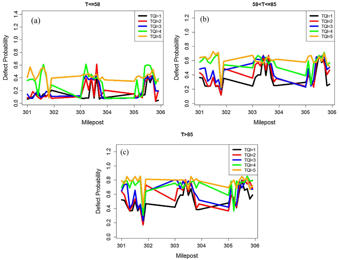
Fig. 6. The probability of geo-defect occurrence under different TQI levels for three inspection intervals; (a)-(c) represent inspection intervals of 0–58 days, 59–85 days, and more than 85 days, respectively.
