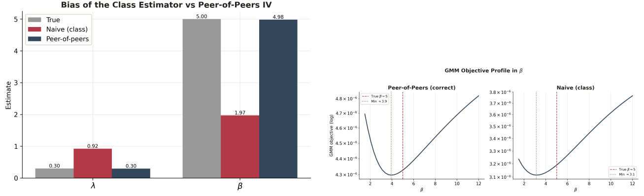
Figure 2. Left: bias of the class estimator vs. the peer-of-peers IV for \lambda and \beta . Right: GMM objective profiles: the correct estimator’s minimum sits at the true \beta = 5 , the naive one at \approx 2 .
