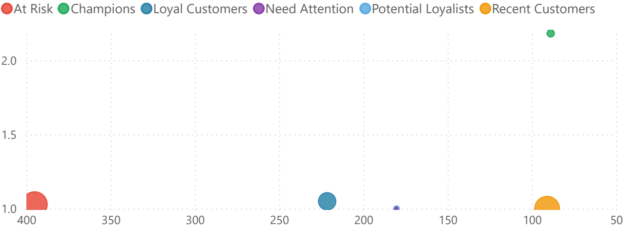
Customer Segments: Recency vs Frequency
