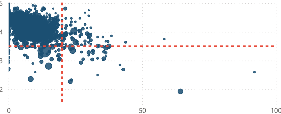
Seller Risk Matrix: Late Rate vs Satisfaction
