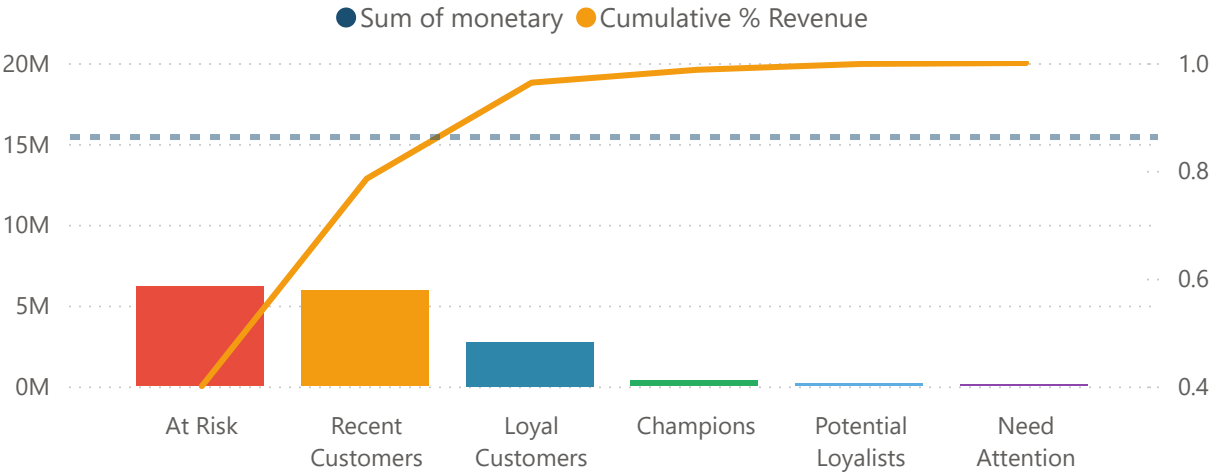
Revenue Concentration by Segment (Pareto Analysis)
