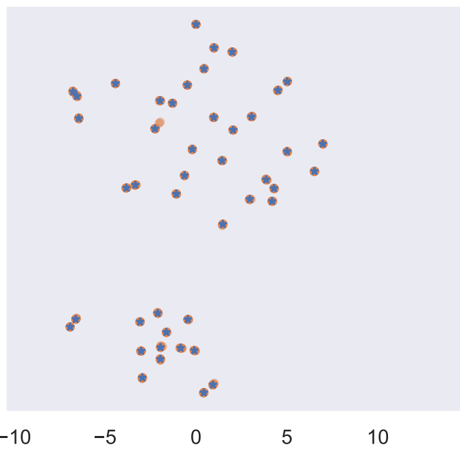
Adding Noise
