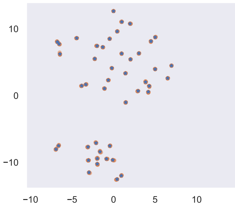
Rephrasing
