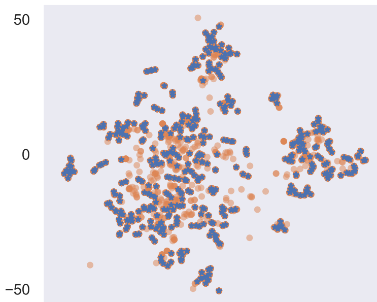
Rephrasing
