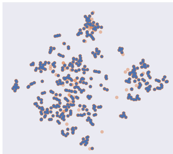
Reordering
