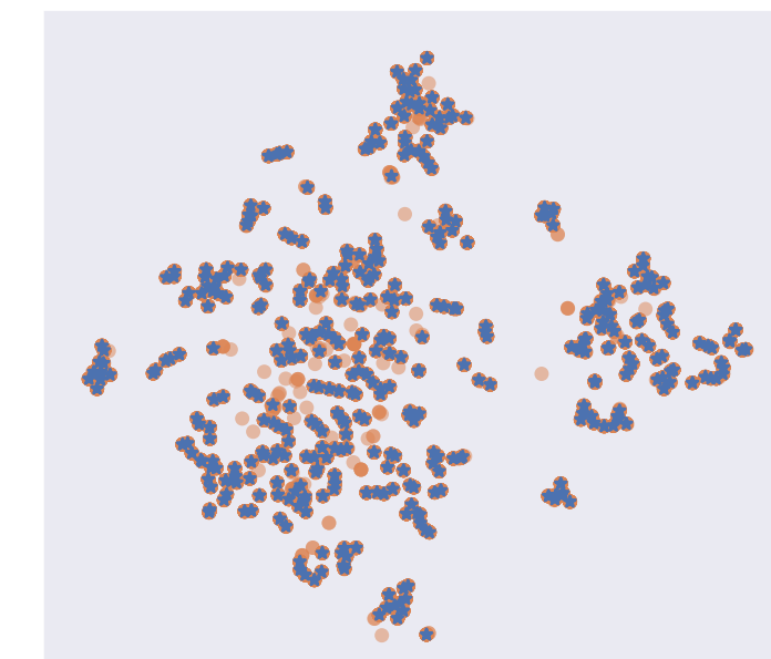
Adding Noise
