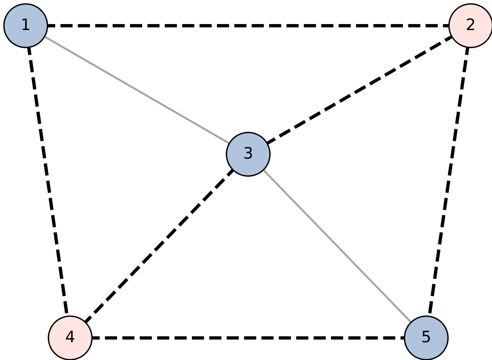
Max-Cut example — cut size: 6
