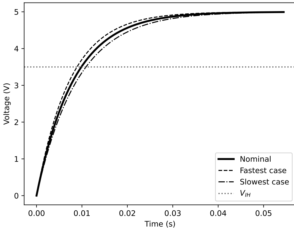
RC Charging with Component Tolerance ( R = 82\text{ k}\Omega , C = 100\text{ nF} )
