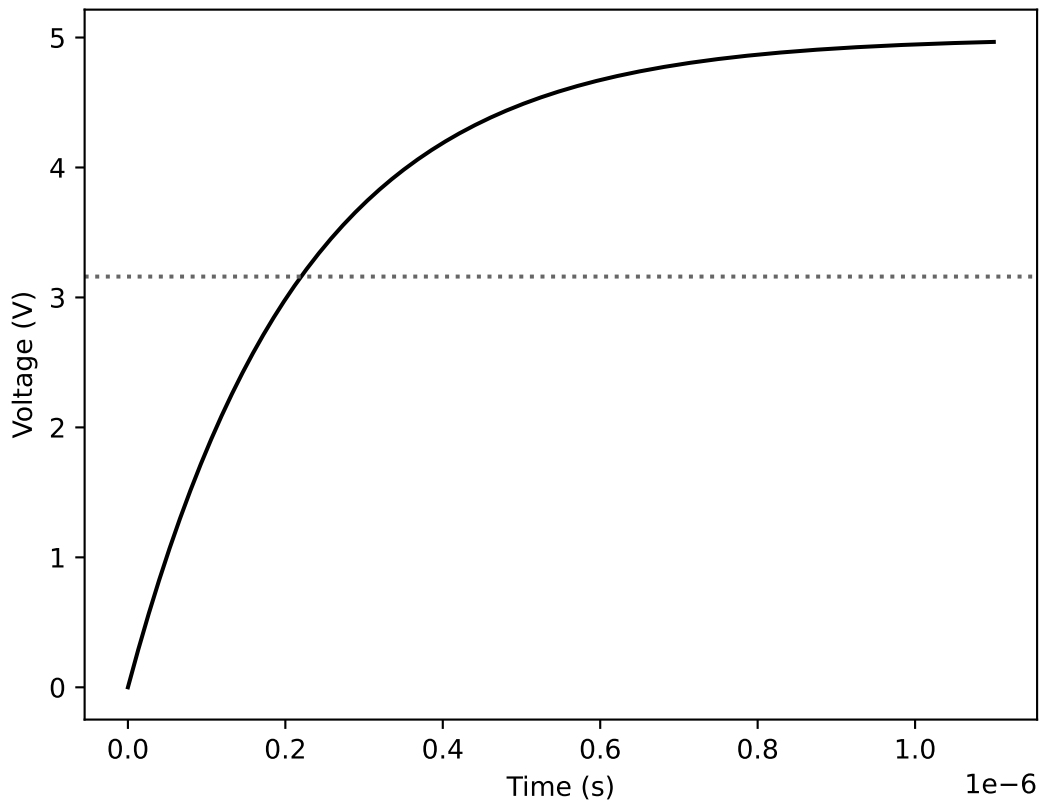
Capacitor charging ( R = 10\text{ k}\Omega , C = 22\text{ pF} )
