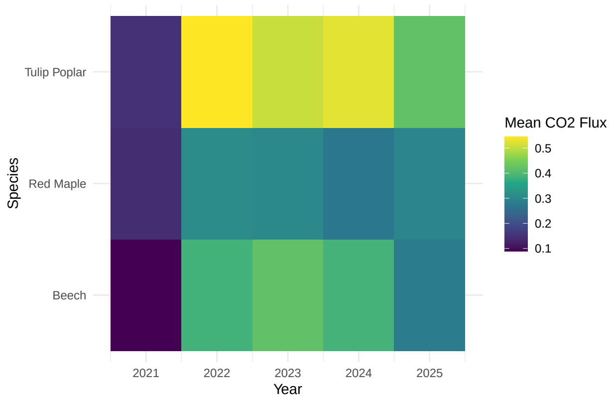
Mean CO2 Flux by Species and Year
