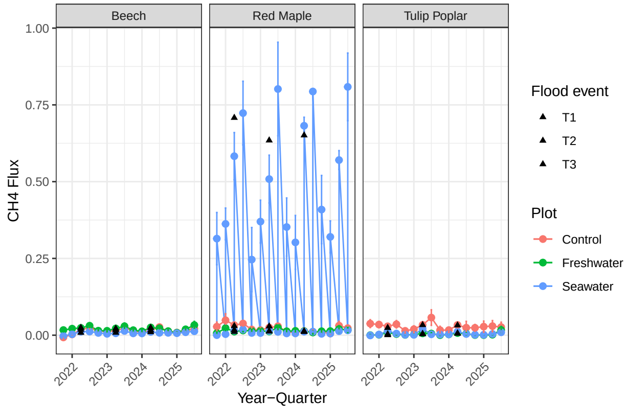
Quarterly CH 4 Flux with Flood Events Highlighted
