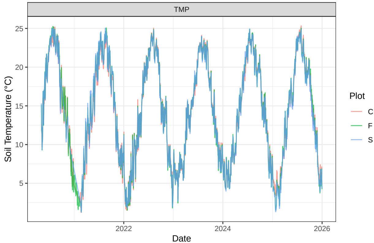
Daily Mean Soil Temperature by Plot
