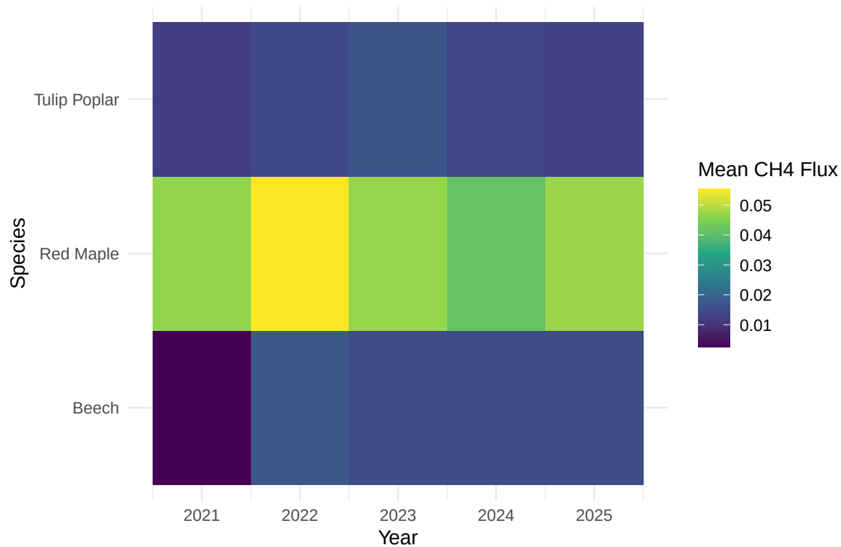
Mean CH 4 Flux by Species and Year
