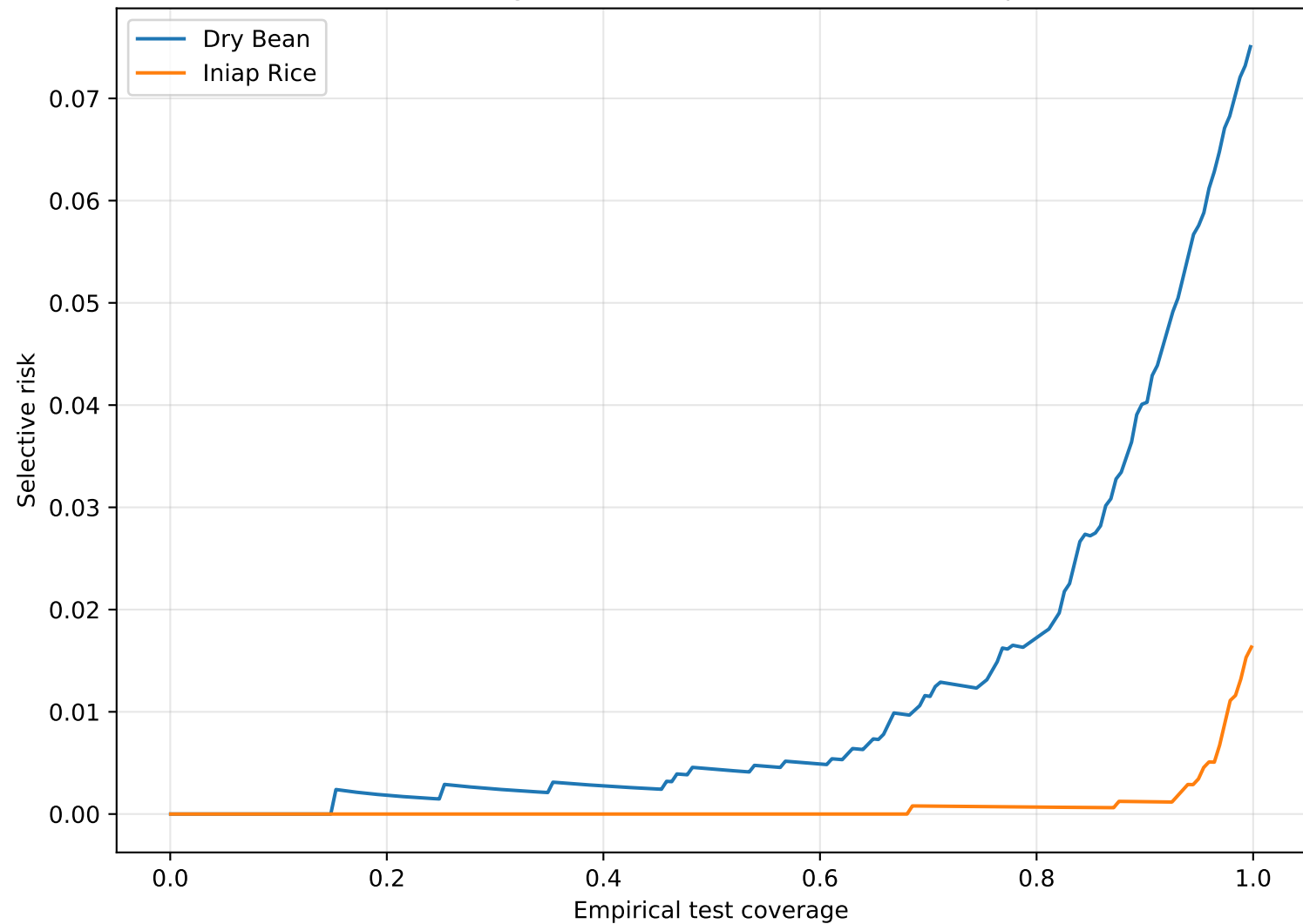
Risk-coverage curves of the exact frozen champions
