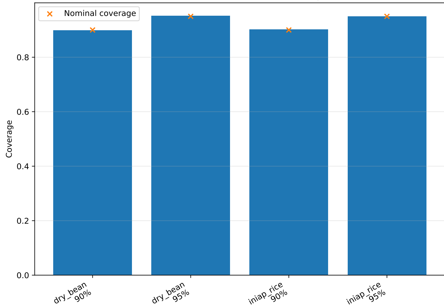
Canonical randomized APS coverage
