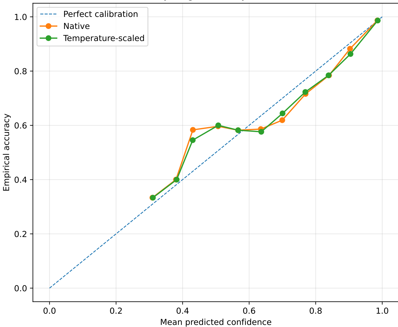
Reliability diagram — Dry Bean — test
