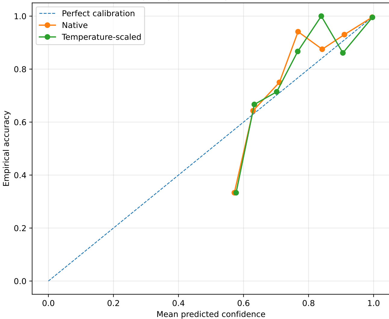
Reliability diagram — Iniap Rice — calibration
