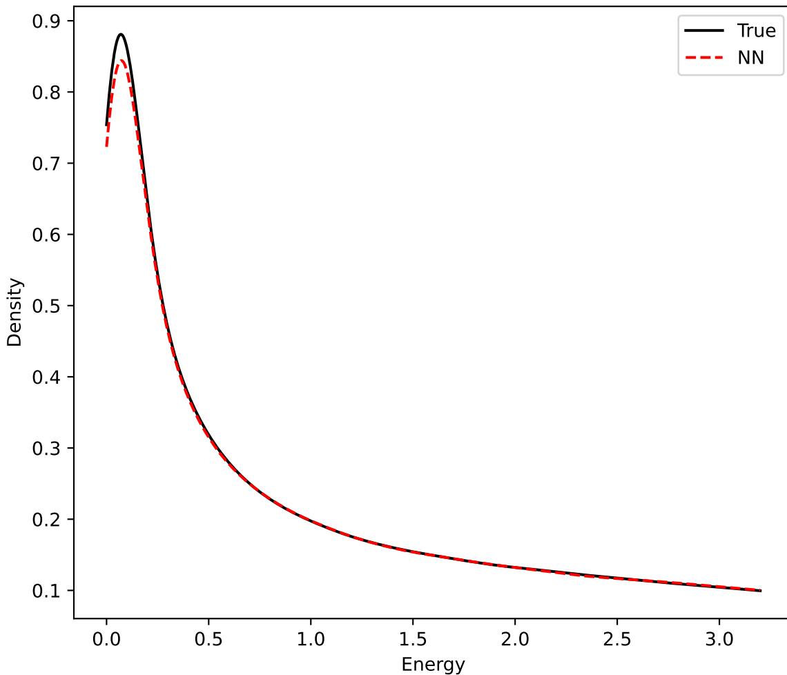
TKE Density Comparison with KS: 0.0088, p-value: 2.8e-77
