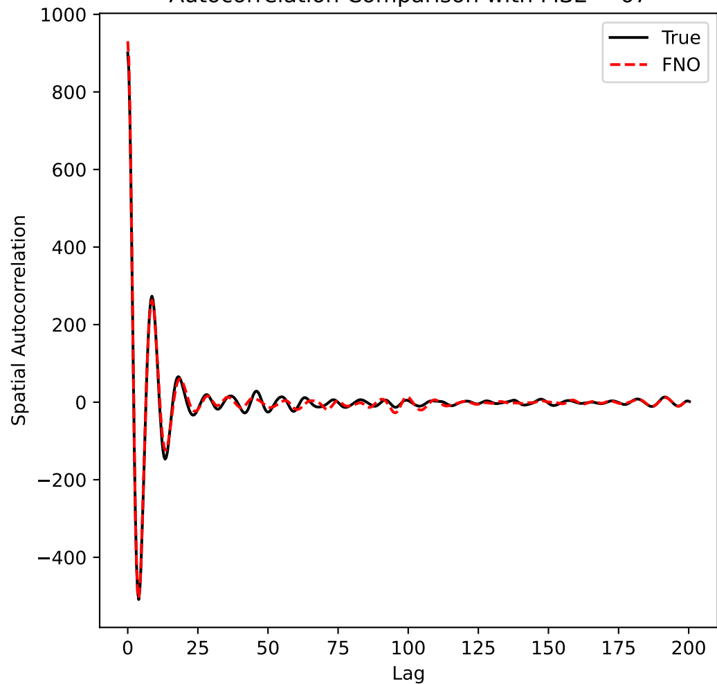
Autocorrelation Comparison with MSE = 67
