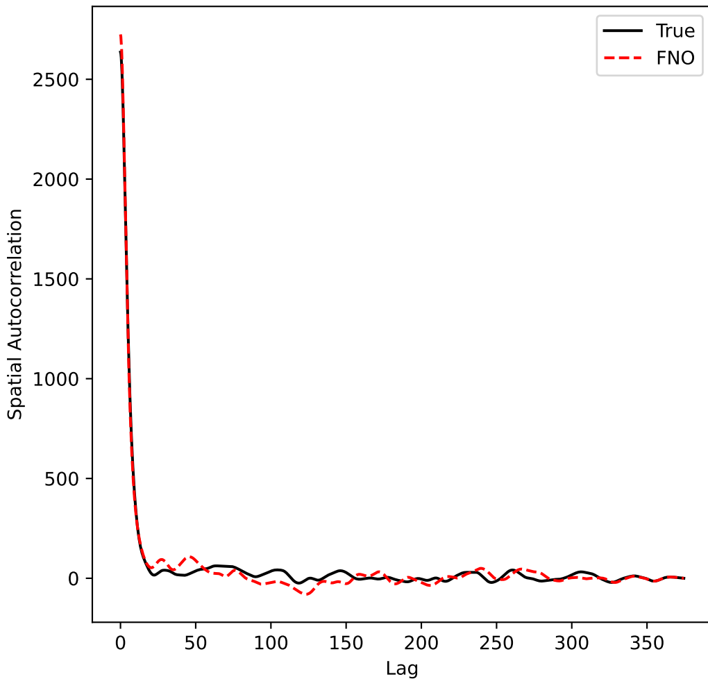
Autocorrelation Comparison with MSE = 1.1\text{e}+03
