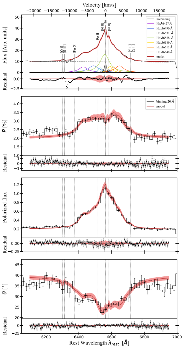
Fig. 2. Spectropolarimetry decomposition of the asymmetric H\alpha profile of 3 C 227. From the top to the bottom, we find the total flux, the degree of polarization ( P ) and the polarized flux (that is the multiplication of the total flux with P ) and the angle of polarization as a function of the rest wavelength in angstrom. The polarized fluxes are shown after binning of 20 Å, while the total flux is displayed without binning. The model fitted to the unbinned data is superimposed on the observations. The residuals, shown under each of the four panels, are calculated relative to the unbinned data on which the fit was performed.
