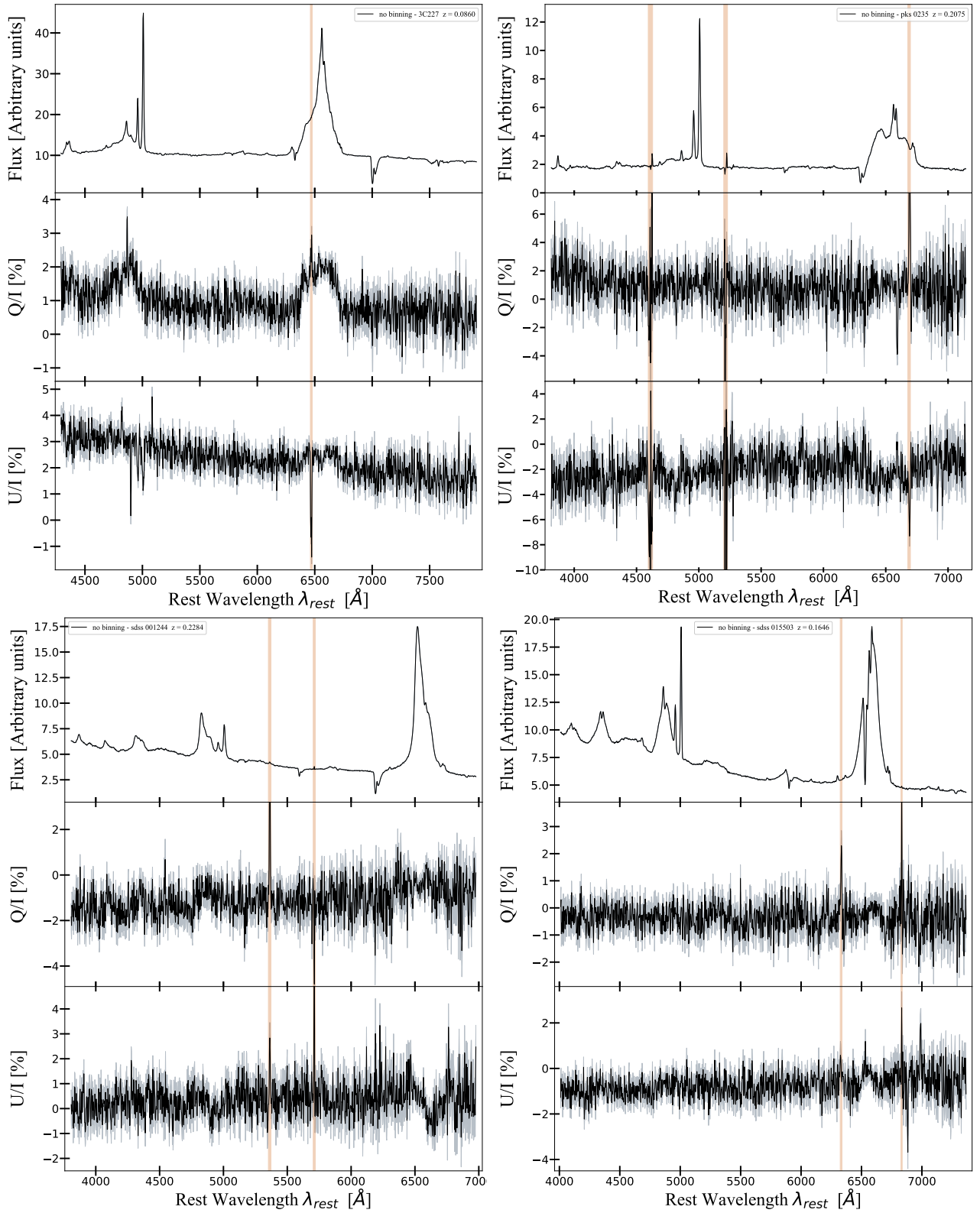
Fig. B.1. Spectra obtained for each observation with FORS2/VLT. Each panel present, from top to bottom, the total flux, and the fraction of Stokes parameters q = Q/I and u = U/I as a function of the wavelength. Top: 3C 227 on the left figure and PKS 0235 for the right figure. Spectral range identified as an artifact and which has been removed are the following: for 3C 227, 6462-6478 Å ; for PKS 0235, 4594-4629 Å, 6676-6698 Å, 5200-5230 Å. Bottom: SDSS 001224, 5352-5373 Å, 5703-5720 Å on the left and SDSS 015530, 6825-6837 Å on the right.
