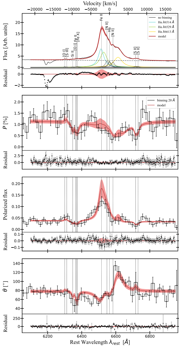
Fig. C.2. Same as 2 but for SDSS 001244
