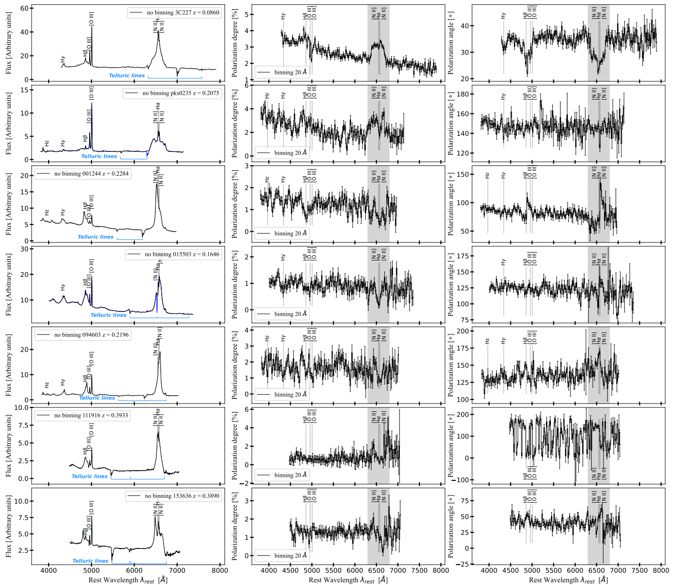
Fig. 1. VLT/FORS2 spectropolarimetry of our sample of seven type 1 AGNs. First column: total flux spectrum (where tellurics are highlighted in blue), second column: polarization degree and third column: angle of polarization as a function of the rest wavelength. The gray zone, in the P and \theta panels, represents the waveband corresponding to the H\alpha profile.
