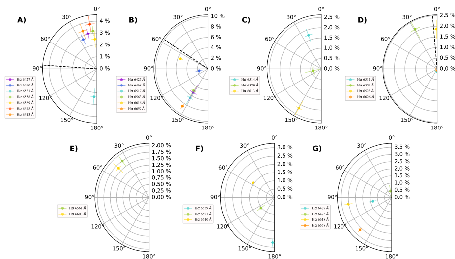
Fig. 3. Protractor diagram of the polarization degree P as a function of the polarization angle \theta for each broad H\alpha component, color-coded as in the spectral decomposition. The polarization angle is measured relative to the celestial north axis, and the radial distance represents P . The black dashed line indicates the radio axis when available: 3C 227 (PA \approx 86^\circ ; Prieto et al. 1993), PKS 0235 (PA \approx 56^\circ estimated from the 1.5 GHz image; Downes et al. 1986), and SDSS 015530 (ENLR PA \sim 5^\circ used as a proxy for the AGN axis; Husemann et al. 2013). Top row: 3C 227, PKS 0235, SDSS 001224, SDSS 015530. Bottom row: SDSS 094603, SDSS 111916, SDSS 153636.
