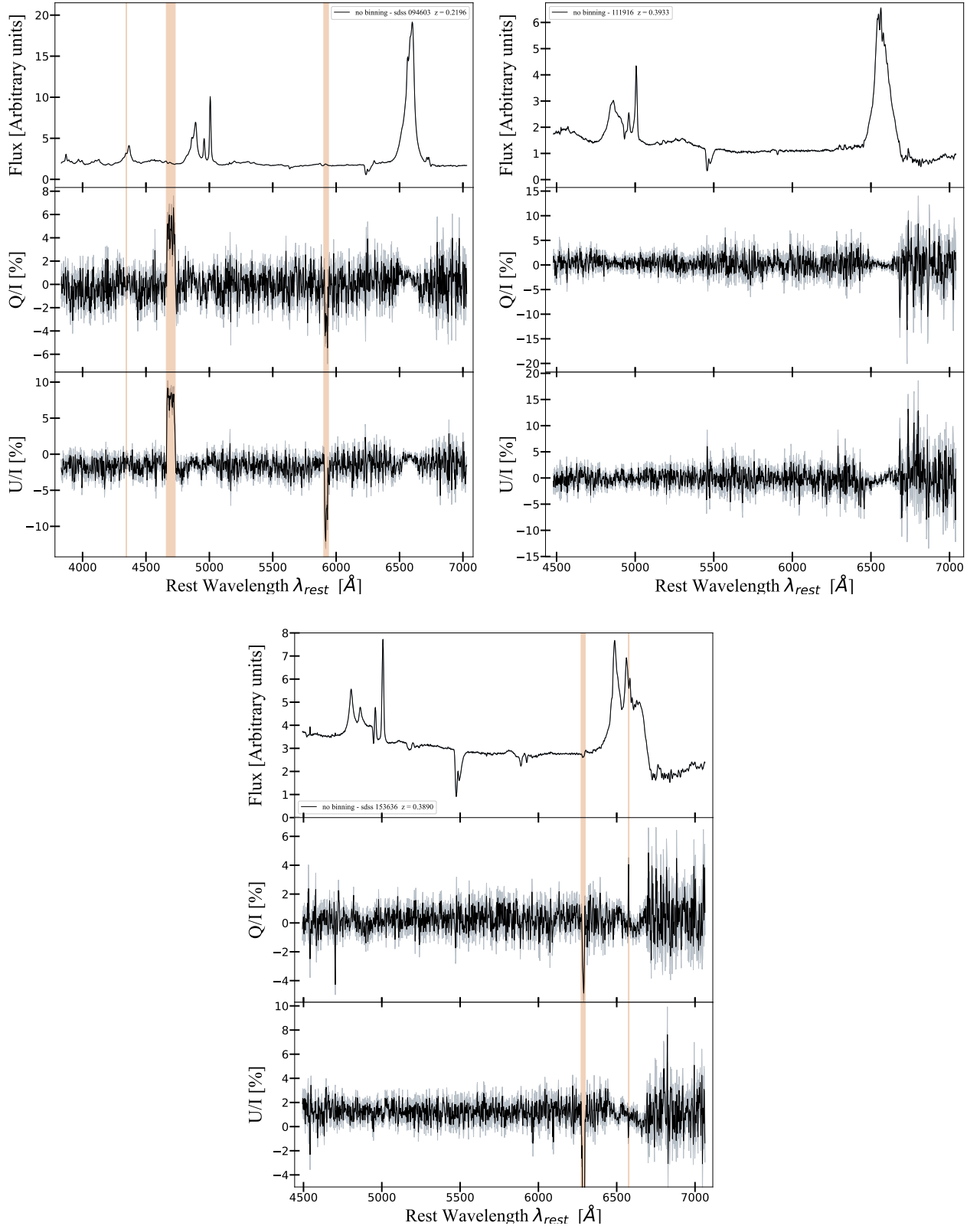
Fig. B.2. Same as B.1, top: SDSS 094603 (left), 4660-4731 Å, 5902-5940 Å and SDSS 111916 (right), bottom: SDSS 153636, 6272-6300 Å, 6573-6579 Å.
