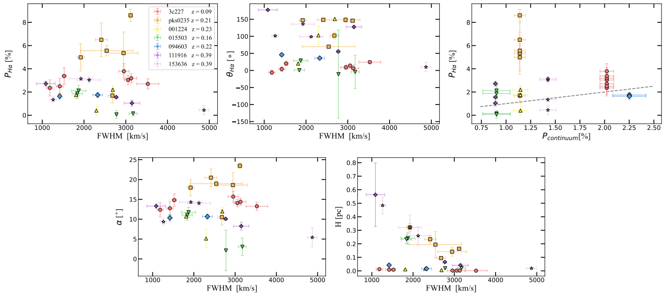
Fig. 4. Geometrical constraints on the BLR inferred from the polarization of the broad H\alpha components. Top row: polarization degree P_{H\alpha} and polarization angle \theta_{H\alpha} as a function of the inferred FWHM, and P_{H\alpha} as a function of the continuum polarization P_{\text{continuum}} . The gray dashed line indicates P_{H\alpha} = P_{\text{continuum}} . Bottom row: effective scattering angle \alpha , and BLR height as a function of the FWHM.
