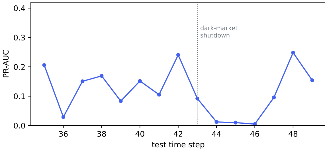
EvolveGCN-O rolling backtest: per-window test PR-AUC
