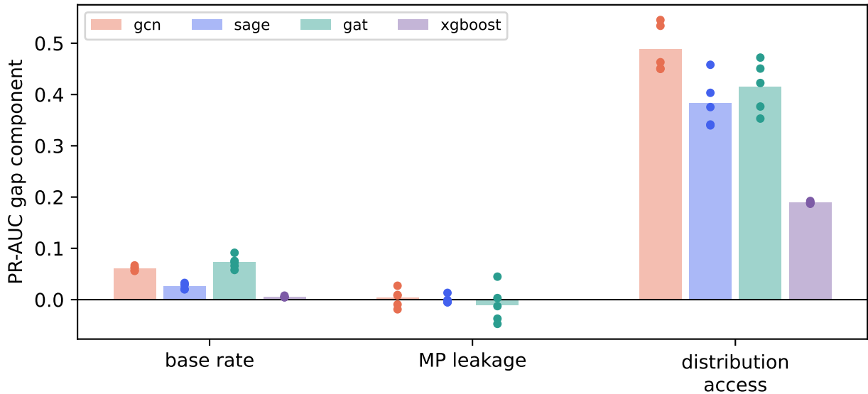
Decomposition of the temporal-vs-random gap (bars = mean, dots = seed)
