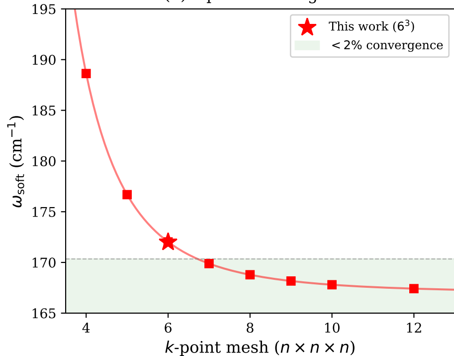
(b) k -point convergence
