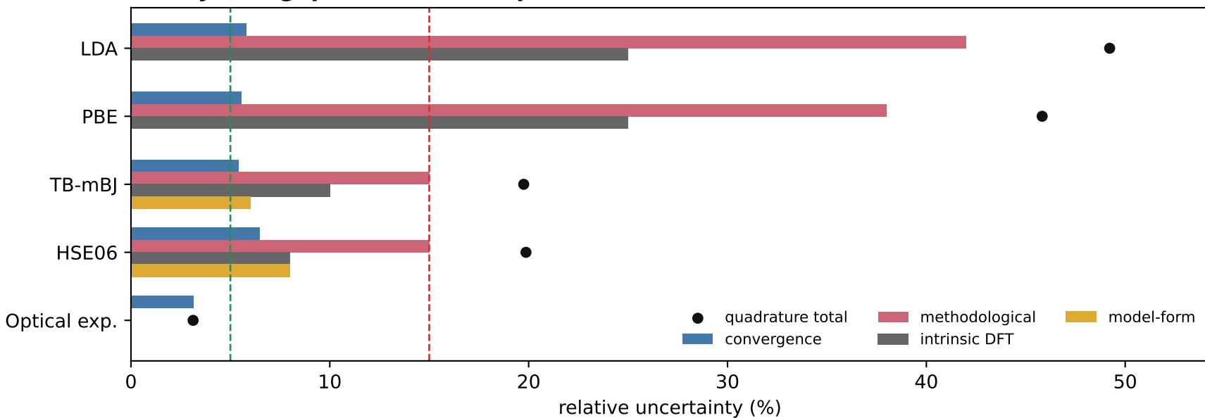
b) Physical-gap certificates expose method-form risk
